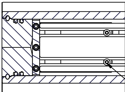
SECTION A-A SCALE .5
