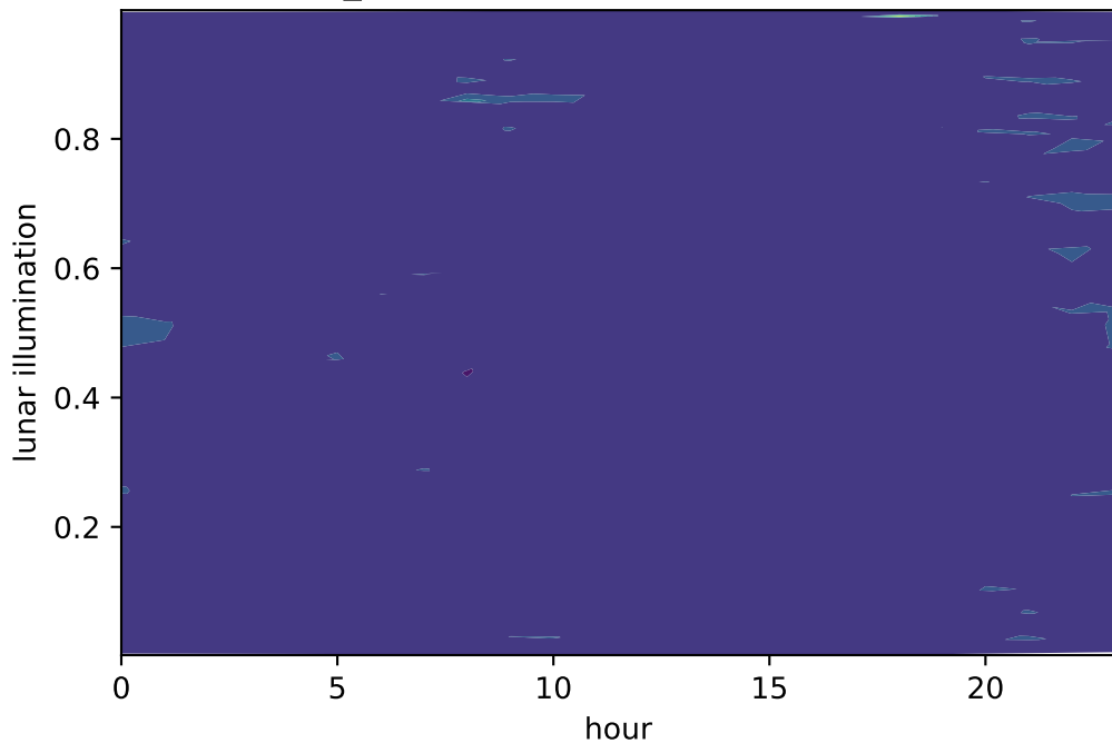
F590_atn by hour and lunar illumination
