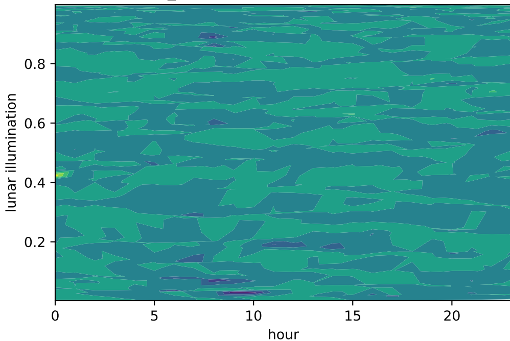
Fd6900_atn by hour and lunar illumination
