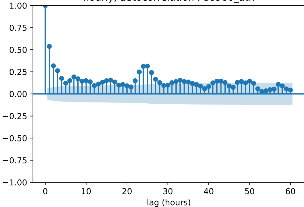
hourly, autocorrelation Fd6900_atn
