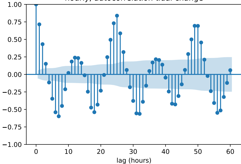
hourly, autocorrelation tidal change
