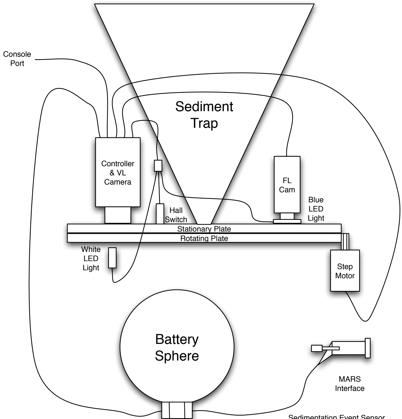
Sedimentation Event Sensor Major Component Interconnections P. McGill 15Mar10
