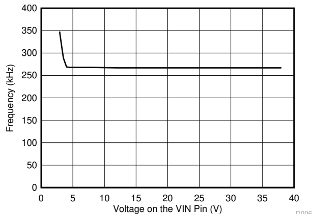
Figure 6-7. Minimum Switching Frequency for Quick Recovery from Frequency Foldback
