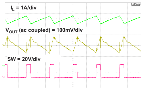
Figure 8-5. CCM PWM Operation
