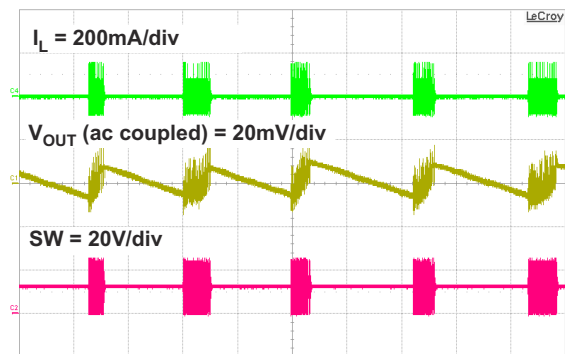
Figure 8-7. Pulse Skipping
