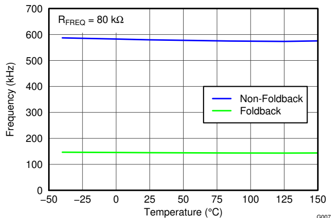
Figure 6-8. Nonfoldback Frequency vs Foldback Frequency
