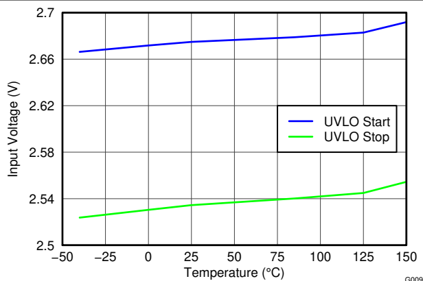
Figure 6-10. Input Voltage UVLO vs Temperature
