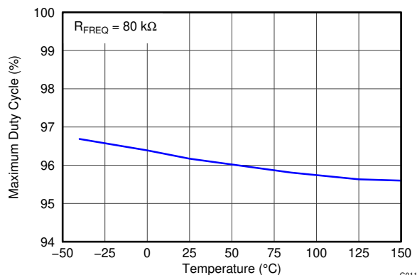
Figure 6-12. Maximum Duty Cycle vs Temperature
