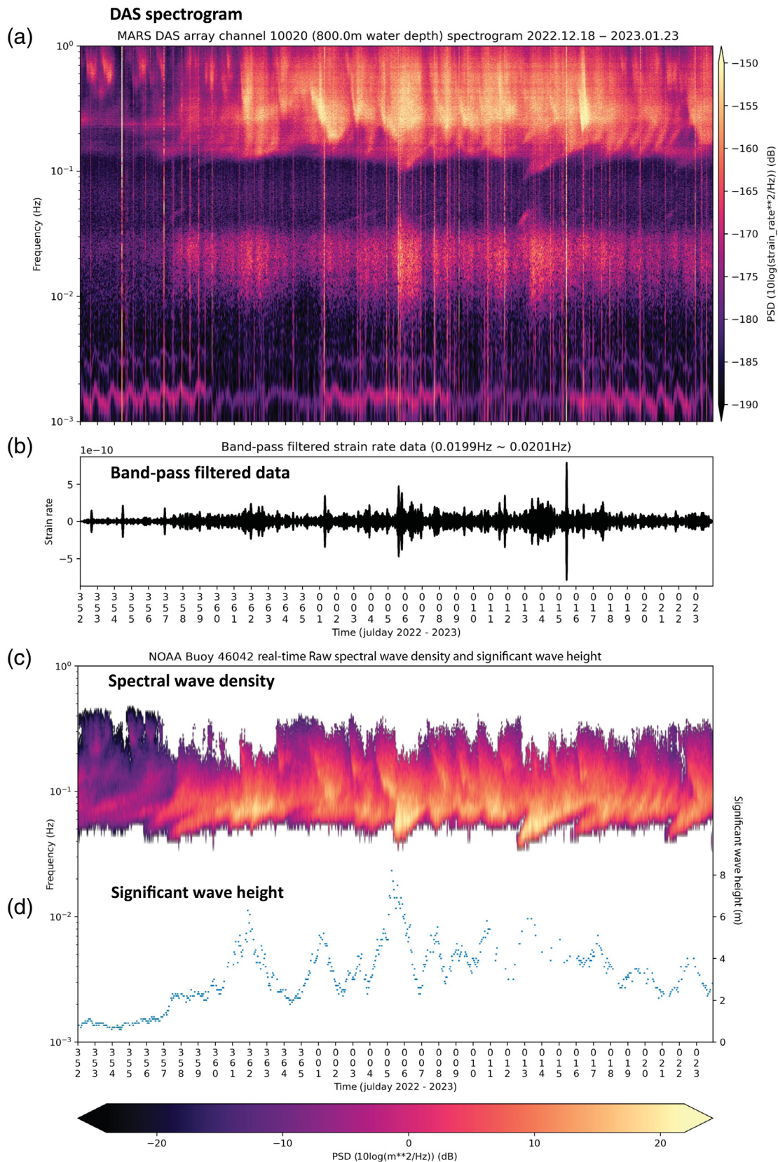
Figure 10. (a) Spectrogram of the DAS recording at channel 10,020 (800 m water depth and 51.1 km along the cable) for Julian day 2022.352–2023.023. (b) Strain rate record, narrow-pass filtered at \sim 0.02 Hz for the same time interval. (c) Spectral wave density (SWD) and (d) significant wave height (SWH) data recorded at NOAA buoy 46,042 (Fig. 1) for the same time
