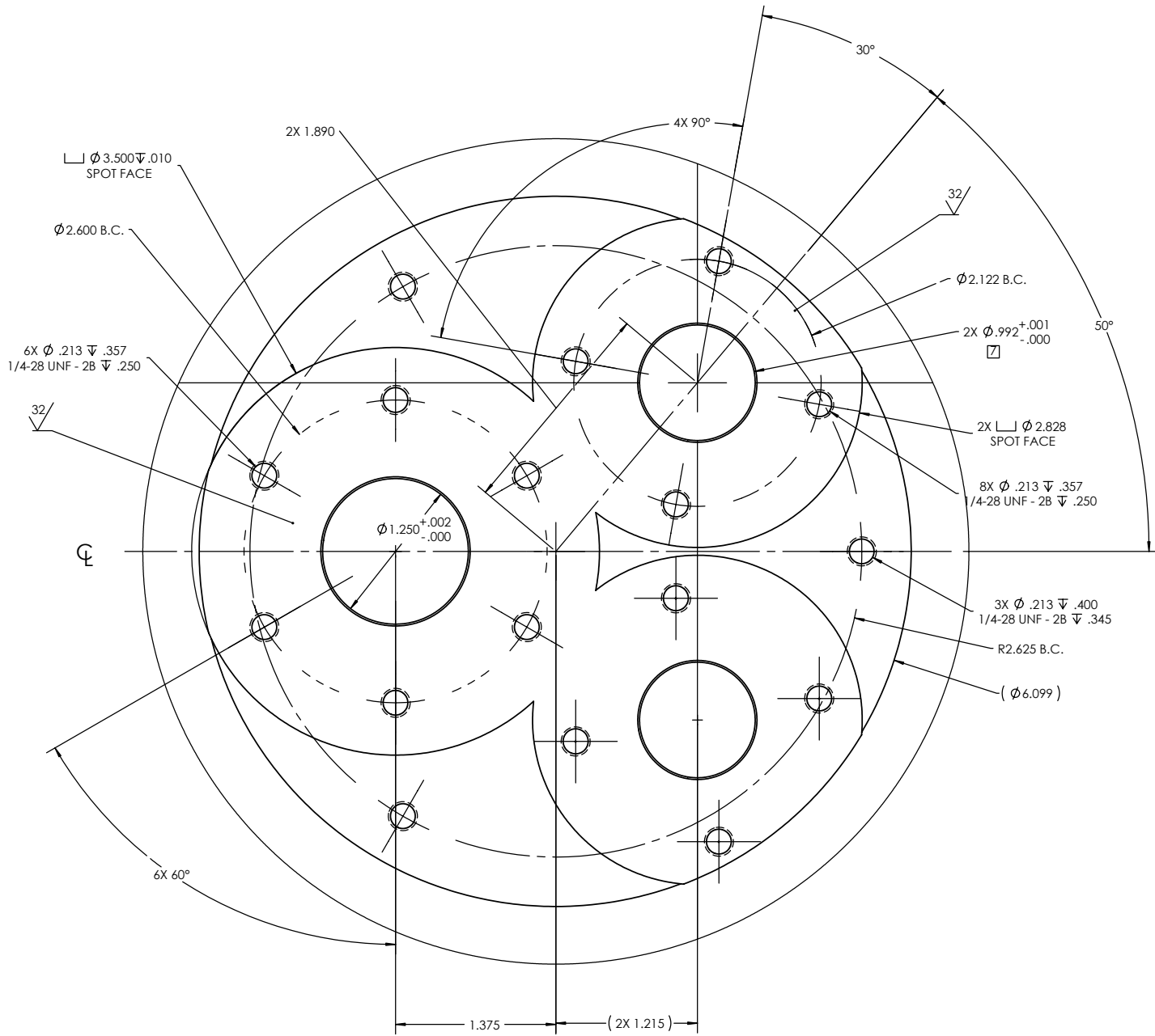
DETAIL D SCALE 1.5 : 1
