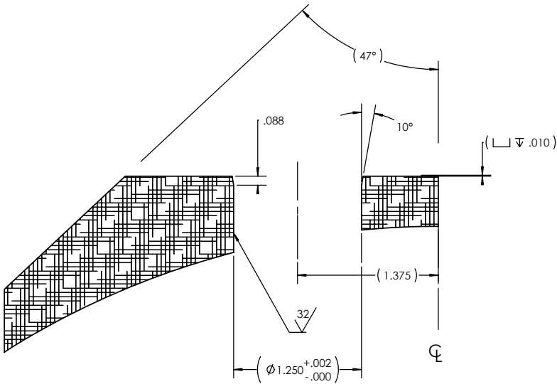
SECTION E-E SCALE 1.5 : 1
