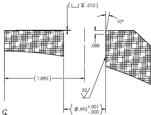
SECTION F-F SCALE 1.5 : 1
