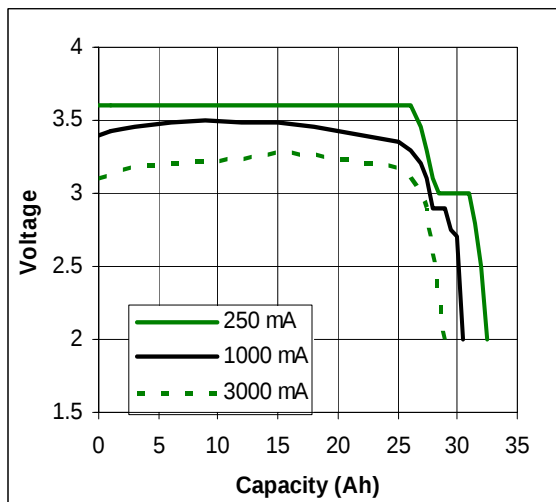
25°C discharge
