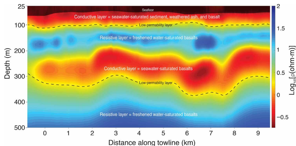
Fig. 3. Line 3 north inversion model. Model showing the electrical resistivity structure of line 3 north (see line location in Figs. 1 and 2). The color scale shows \log_{10}[\rho(\text{ohm-m})] . This multilayer inversion model is composed of four lateral formations: two conductive seawater-saturated basalt layers intermitted by two resistive freshened water-saturated basalts. Low-permeability thin horizons of ash/soil (dashed lines) separate the conductive and resistive layers. The model was derived from the data acquired by three surface-towed CSEM receivers at 3 and 7 Hz. Inversion error floors include amplitude, 7%, and phase, 4%.
