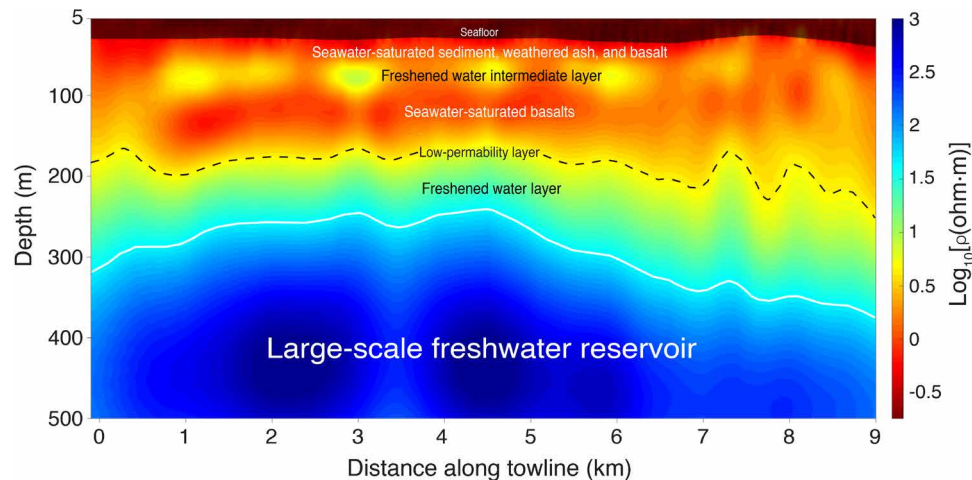
Fig. 4. Line 2 south inversion model. Model showing the electrical resistivity structure of line 2 south (see line location in Figs. 1 and 2). The color scale shows \log_{10}[\rho(\text{ohm-m})] . The deep and laterally continuous resistive body ( \sim 1000 ohm-m) represents a large-scale freshwater reservoir (area bounded by a white line). A low-permeability thin layer (black dashed line) separates between the upper seawater-saturated (resistivity of \sim 1 to 3 ohm-m) basalts and the freshened water layer ( \sim 5 to 50 ohm-m) situated between \sim 190 - to 320 -m depths. A moderately resistive body ( \sim 5 to 10 ohm-m) exists between \sim 60 - to 100 -m depths, interpreted as an intermediate layer of freshened water. The conductive layer beneath the seafloor ( \sim 30 - to 50 -m depth) indicates seawater-saturated sediment, weathered ash, and basalts. The model was derived from the data acquired by four surface-towed CSEM receivers at 3 and 7 Hz. Inversion error floors include amplitude, 7\% , and phase, 4\% . This inversion converged to an RMS misfit of 0.99 after eight iterations. The model-to-data fits and normalized residuals are shown in fig. S4.
