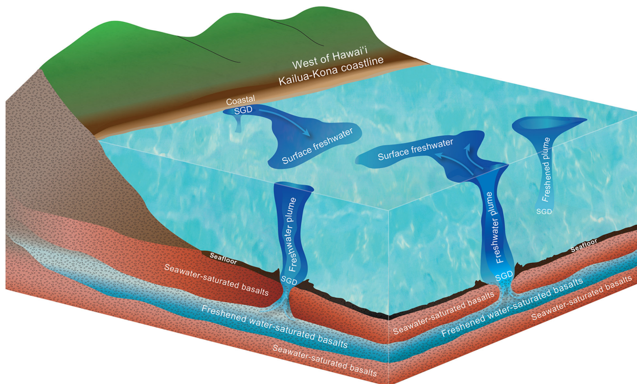
Figure 4. Conceptual model illustrating freshwater plumes and surface freshwater systems offshore west Hawai'i. Fresh groundwaters are transported from onshore to offshore through multilayer basaltic formation (Attias et al., 2020). From this sub-seafloor formation, freshened/freshwater migrate upward via porous/fractured seawater-saturated basalts, producing multiple large-scale vertical plumes that extend from the seafloor to the ocean surface. Surface freshwater bodies disconnected from plumes most likely result from nearby seeps or coastal SGD runoffs.
