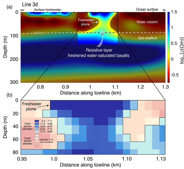
Figure 3. (a) Two-dimensional inversion model derived from the CSEM data acquired in survey line 3d. The color scale presents the electrical resistivity in \log_{10}[\rho(\Omega\text{m})] . The gray dashed line represents the seafloor, positioned at a water depth of \sim 95 m. For enhanced visibility of the water column resistive anomalies, the resistivity shading thresholds are \sim 1.7 \Omega\text{m} and \sim 6 \Omega\text{m} for the plume and surface freshwater body, respectively. Distinctive freshwater plume imaged at a towline distance of \sim 1 – 1.1 km. This inversion converged to an RMS of 1.0 after 15 iterations, with error floors of 9% (amplitude) and 7% (phase) data. Black rectangular represents the water column plume area selected for salinity calculation. (b) Line 3d water column salinity distribution. The black line encompasses low salinities ( <10 ) within the plume, calculated from the resistivity model. The average plume salinity is 4.4, with \sim 87\% of freshwater. Salinities outside the plume were not calculated (see Section 2.3).
