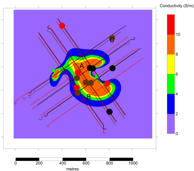
Fig. 9: Plan map view of a 3D model of the inverted CSEM conductivity at a depth of 1632 mbsf. The 2 green triangles are the transmitter positions, while the locations of the ORP minima for the entire survey are plotted as black circles for circuit 1, brown circles for circuit 2, and red circles for circuit 3.
