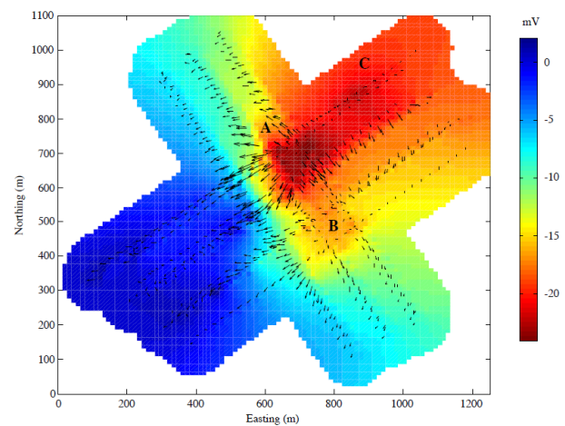
Fig. 10: Self potential derived from E_x and E_y data shown in Fig. 6 by Occam's inversion. Arrows show the directions of the potential differences as measured by the AUV CSEM system, scaled by amplitude.
