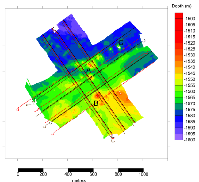
Fig. 5: Bathymetry map of the test area derived from circuit 1 multibeam bathymetry data. AUV tracks from circuit 1 (black), circuit 2 (brown), and circuit 3 (red) are shown. Labels A-C show area of anomalous self-potential.
