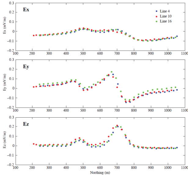
Fig. 6: 30 second averages of the electric field data, after levelling, for the eastern most lines of the southeast-northwest lines of the three repeated circuits.
