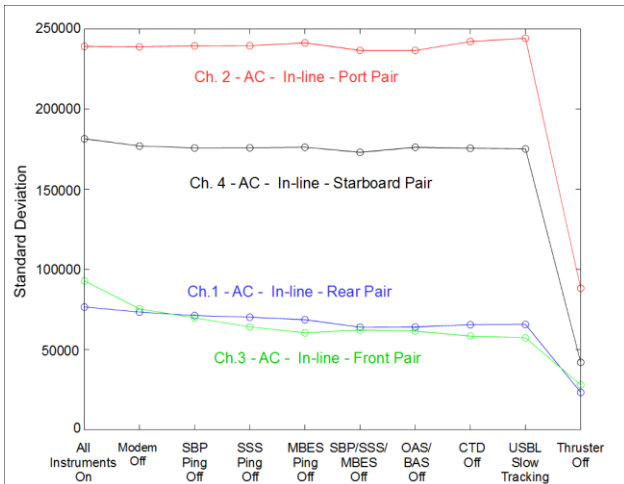
Fig. 2: The noise levels on the AC channels as the payload equipment was successively turned off, with the actions indicated on the bottom axis. The noise level with all the equipment on is only slightly higher than most of the equipment turned off. Turning the vehicle motor off was the only action that substantially decreased the noise level, indicating the primary noise source was related to the thruster.
