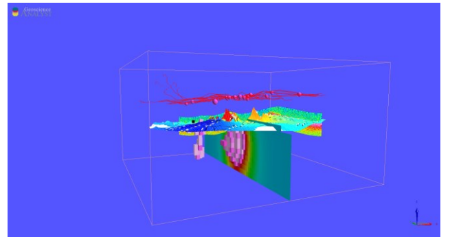
Fig. 7: 3-D data model of the AUV-CSEM data. On the top layer are the AUV tracks and the locations of the ORP minima (pink spheres). The SP inversion result from Fig. 10 is painted on the multibeam bathymetry (vertical exaggeration 2x). Beneath the seafloor surface, a subbottom profile is displayed. The inverted conductivity model derived from the CSEM data is displayed as both a vertical slice through the model and an isosurface. The volume is approximately 1100m x 1200m x 250m.
