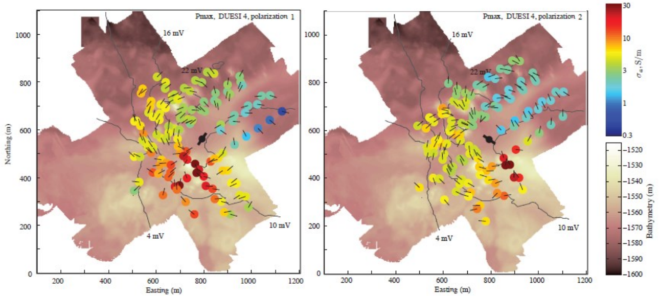
Fig. 8: Apparent conductivity (colored disks – log10 scale) overlain on bathymetry for two polarizations of CSEM transmission from a deployed transmitter (center black symbol). For this example, the transmission frequency is 14 Hz, and the black lines show the directions of the polarization ellipse maxima recorded by the AUV.
