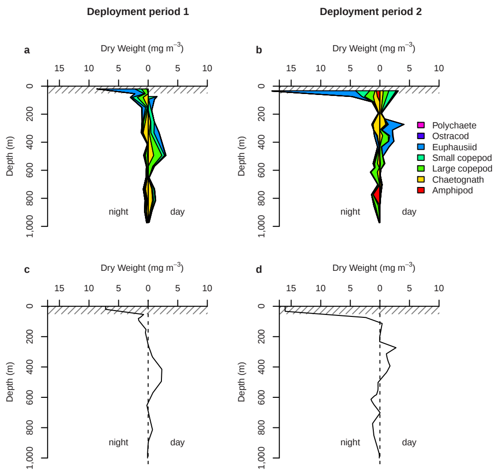
Extended Data Figure 3 | Zooplankton depth distribution.
