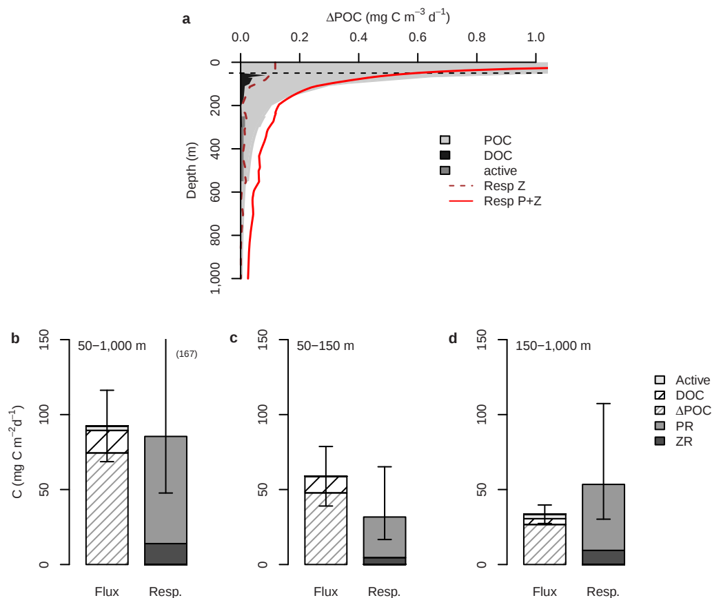
Extended Data Figure 5 | Twilight-zone carbon budget with different depth horizons. a , Organic matter supply via dissolved matter (black area), active transport (mid grey area) and total supply including particles (light grey area), compared with zooplankton respiration (dashed red line) and community respiration (prokaryotes plus zooplankton; solid red line). b–d , Comparison of
