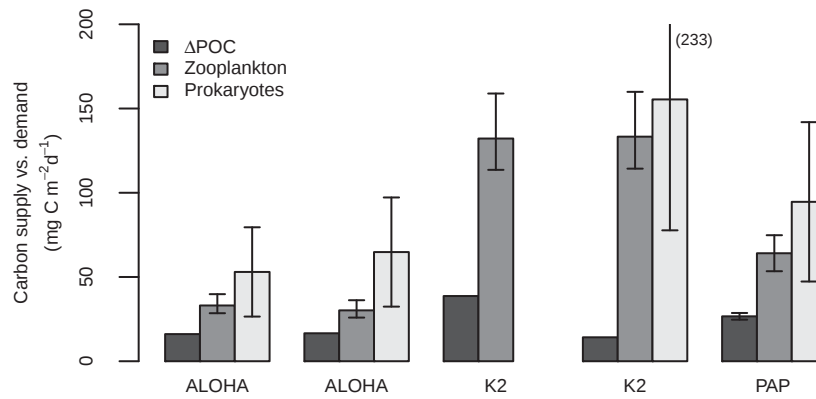
Extended Data Figure 8 | Twilight-zone carbon budgets based on ‘carbon demand’. Budgets were compiled by comparing loss of POC ( \Delta POC; black) with carbon demand (ingestion) by zooplankton (dark grey) and prokaryotes (light grey) in the North Atlantic (PAP; this study) and twice at each of two stations in the Pacific (ALOHA and K2; ref. 6). The imbalance of these budgets
