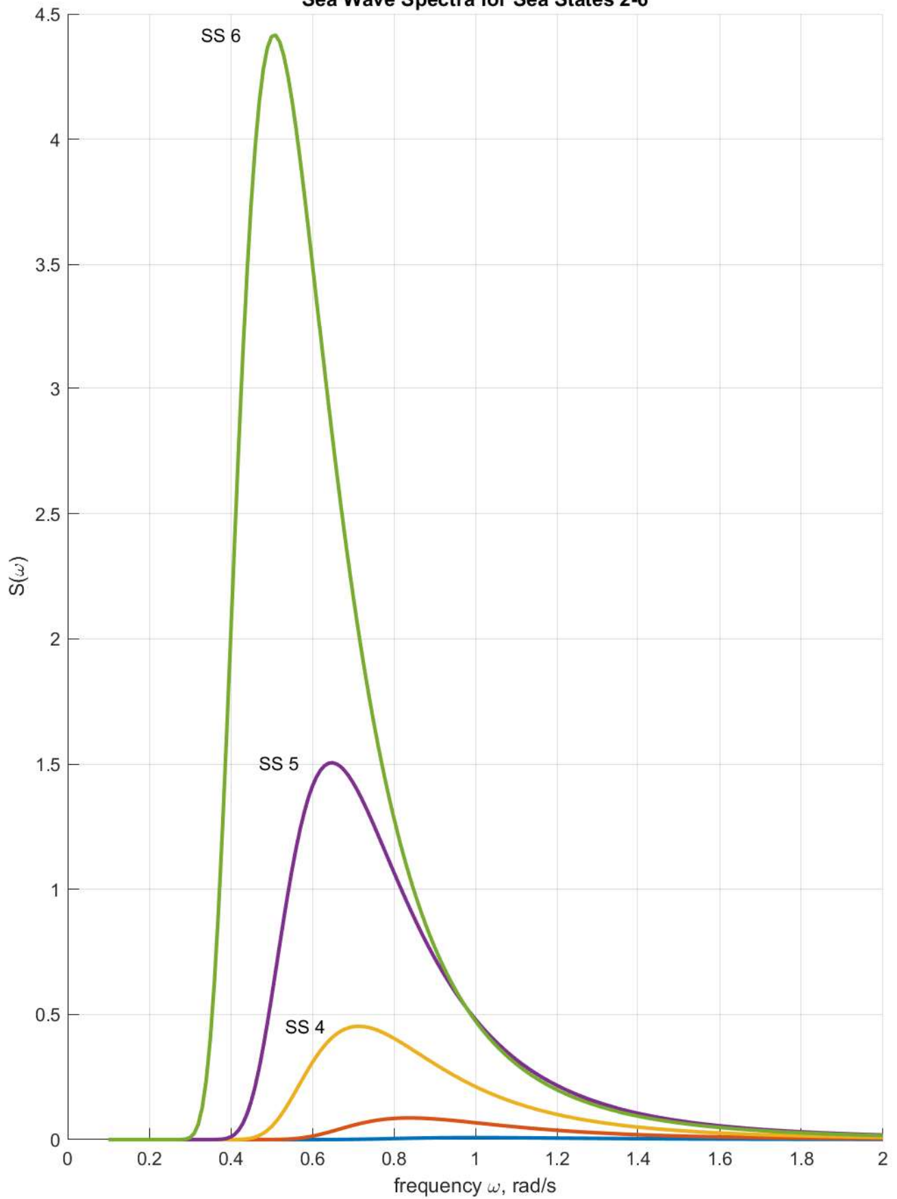
Sea Wave Spectra for Sea States 2-6
