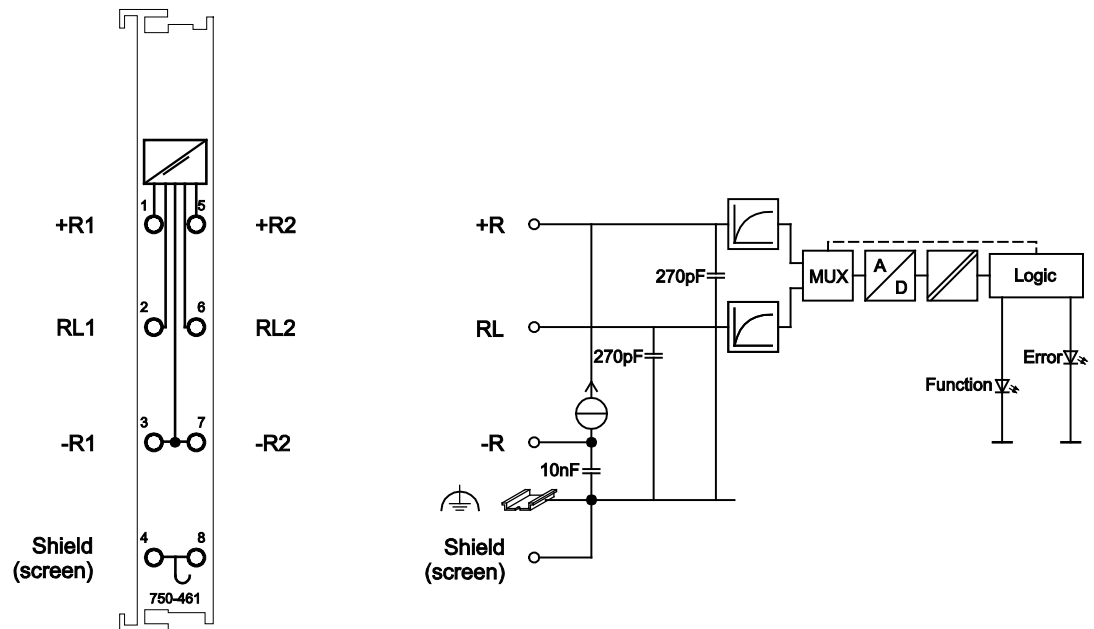
Figure 5: Schematic Diagram
