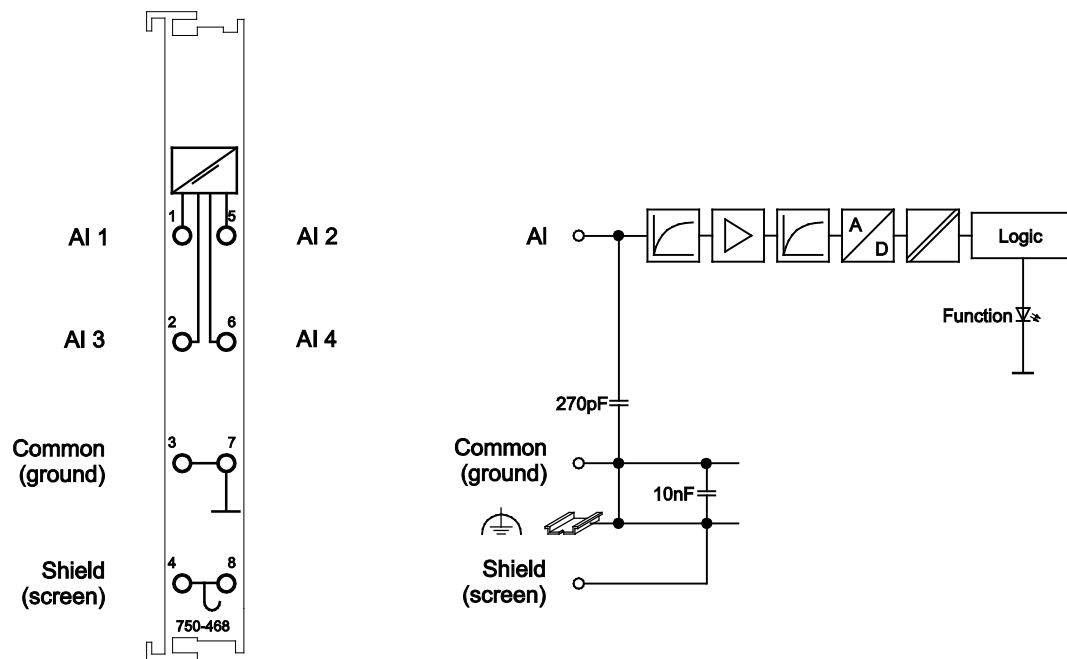
Figure 5: Schematic Diagram
