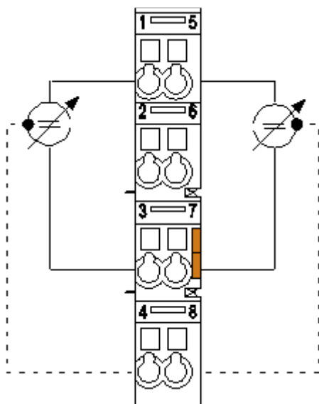
Figure 11: Connection Example – 2-Wire 0 V
