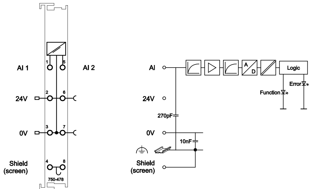
Figure 6: Schematic Diagram
