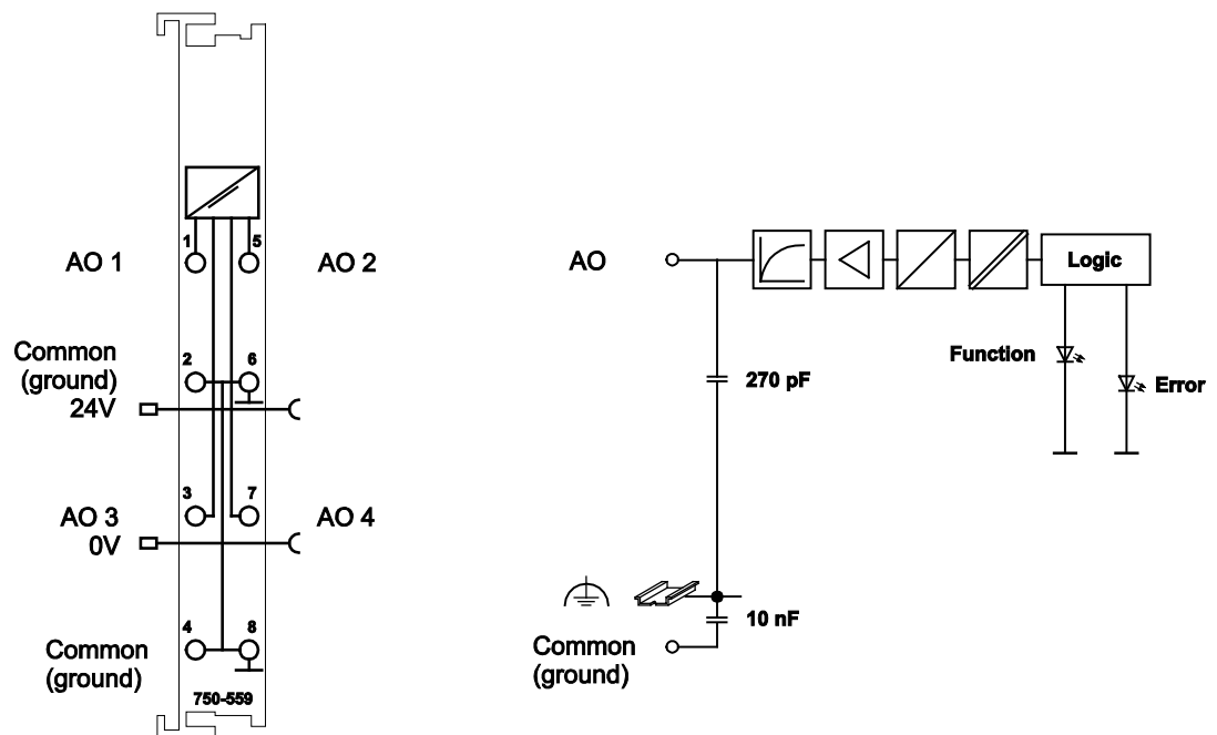
Figure 6: Schematic Diagram
