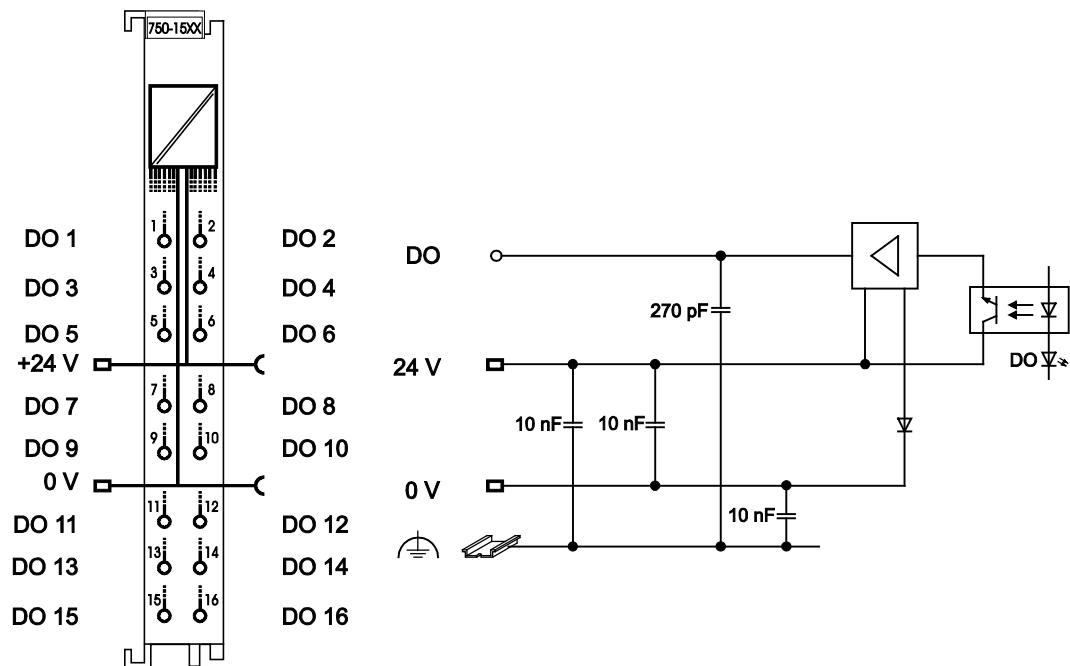
Figure 6: Schematic Diagram
