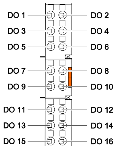
Figure 4: CAGE CLAMP® S Connectors
