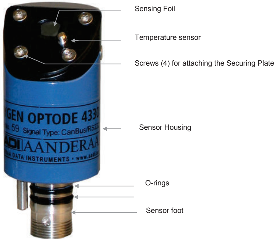
Figure 1-1 Illustration of the Oxygen Optode 4330.
