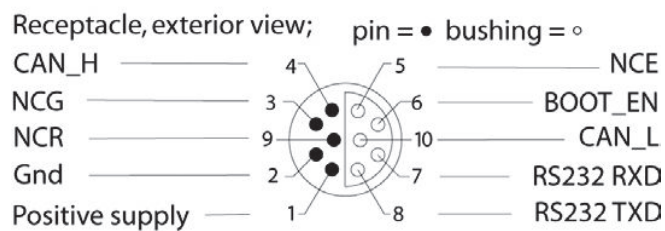
Figure 1-1A Oxygen Optode 4330 Pin Configuration
