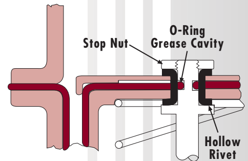
Fig. 39: Slip Joint Shaft Assembly
