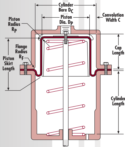
Fig. 17: Hardware Dimensions
