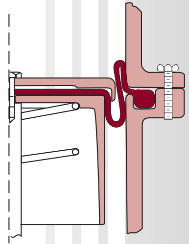
Fig. 38: Pressure Reversal of Diaphragm
