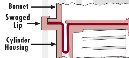
Fig. 22: Swaged Lip
