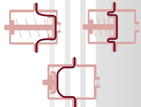
Fig. 13: Involute Diaphragm cycle. Convolution is not required at stroke limits.
