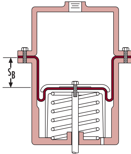
Fig. 6: Down-Stroke Position
