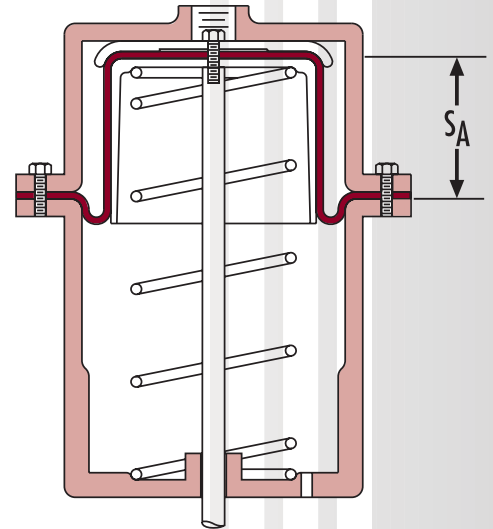
Fig. 7: Up-Stroke Position
