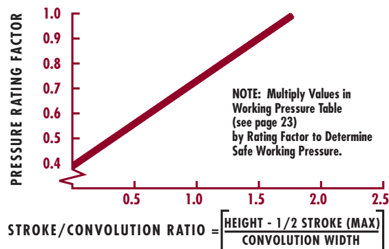
Fig. 16: Pressure rating graph
