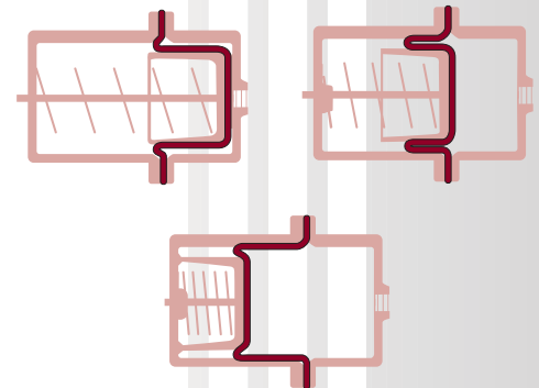
Fig. 12: Standard rolling diaphragm cycle. Convolution is present at all times.
