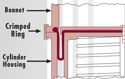
Fig. 29: Crimped Ring
