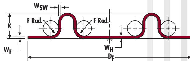
Fig. 10: Preconvoluted Diaphragm
