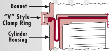
Fig. 25: Ring Clamp
