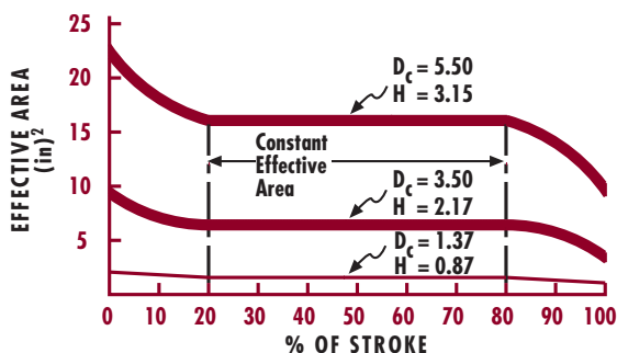
Fig. 15: Force output curve
