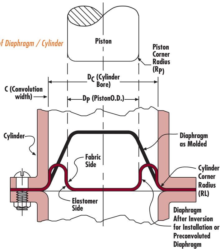
Fig. 6: Down-Stroke Position
