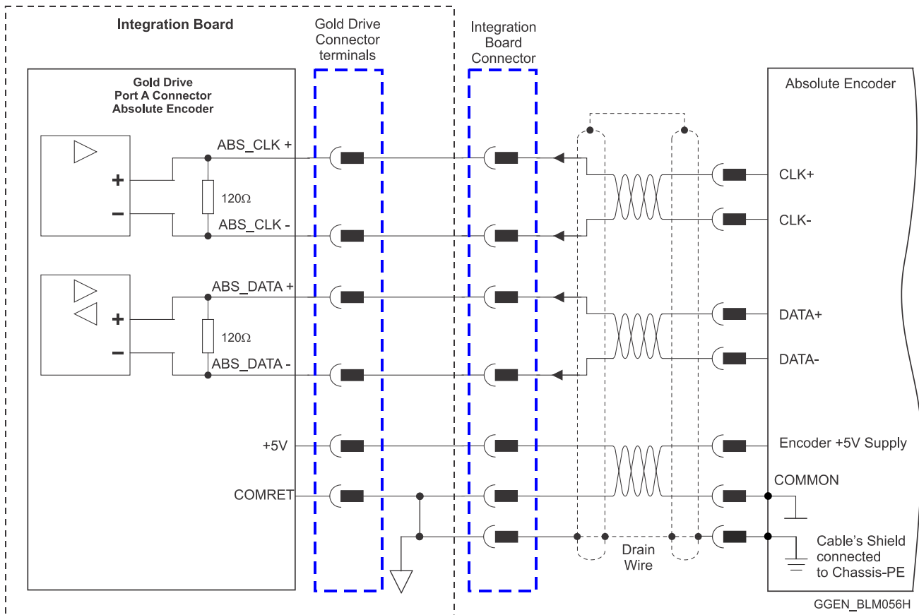
Figure 28: Absolute Serial Encoder – Recommended Connection Diagram for Endat, Biss, SSI
