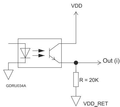
Figure 47: Digital Output TTL Schematic
