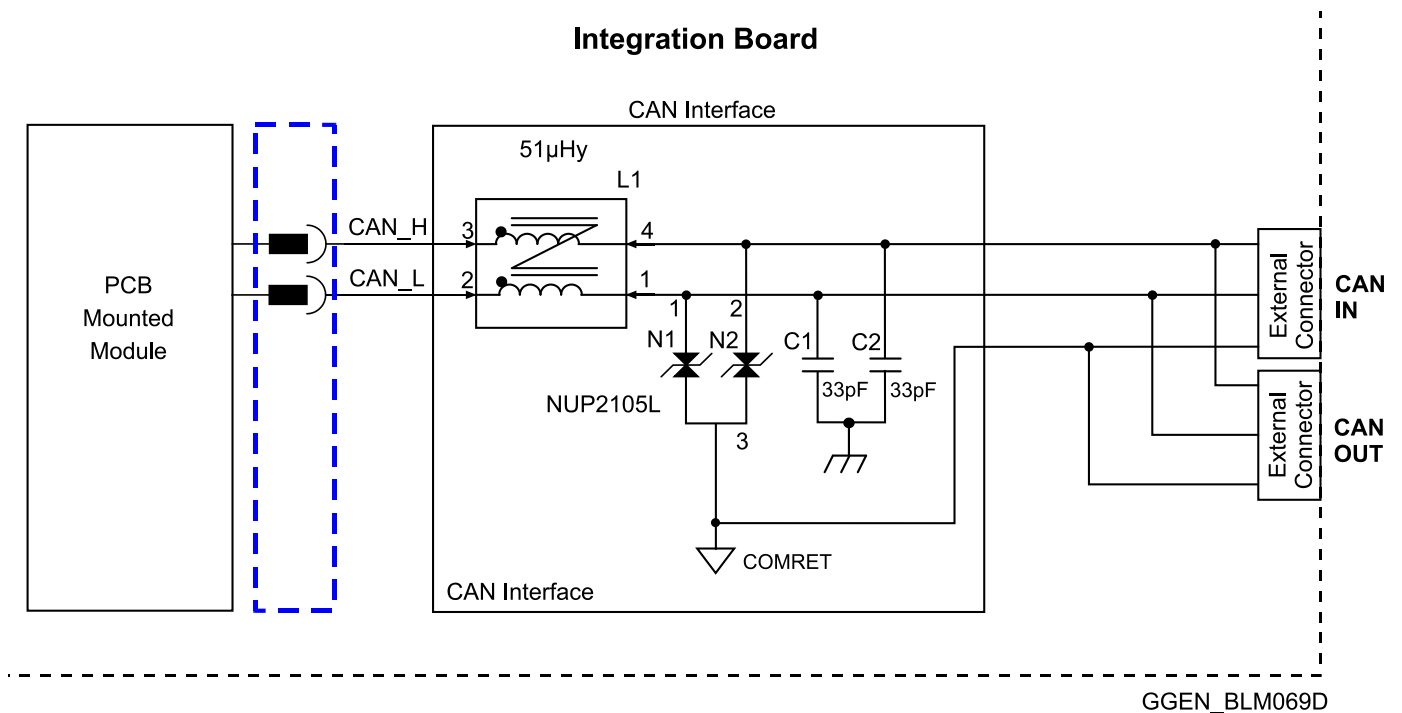
Figure 63: CAN Interface
