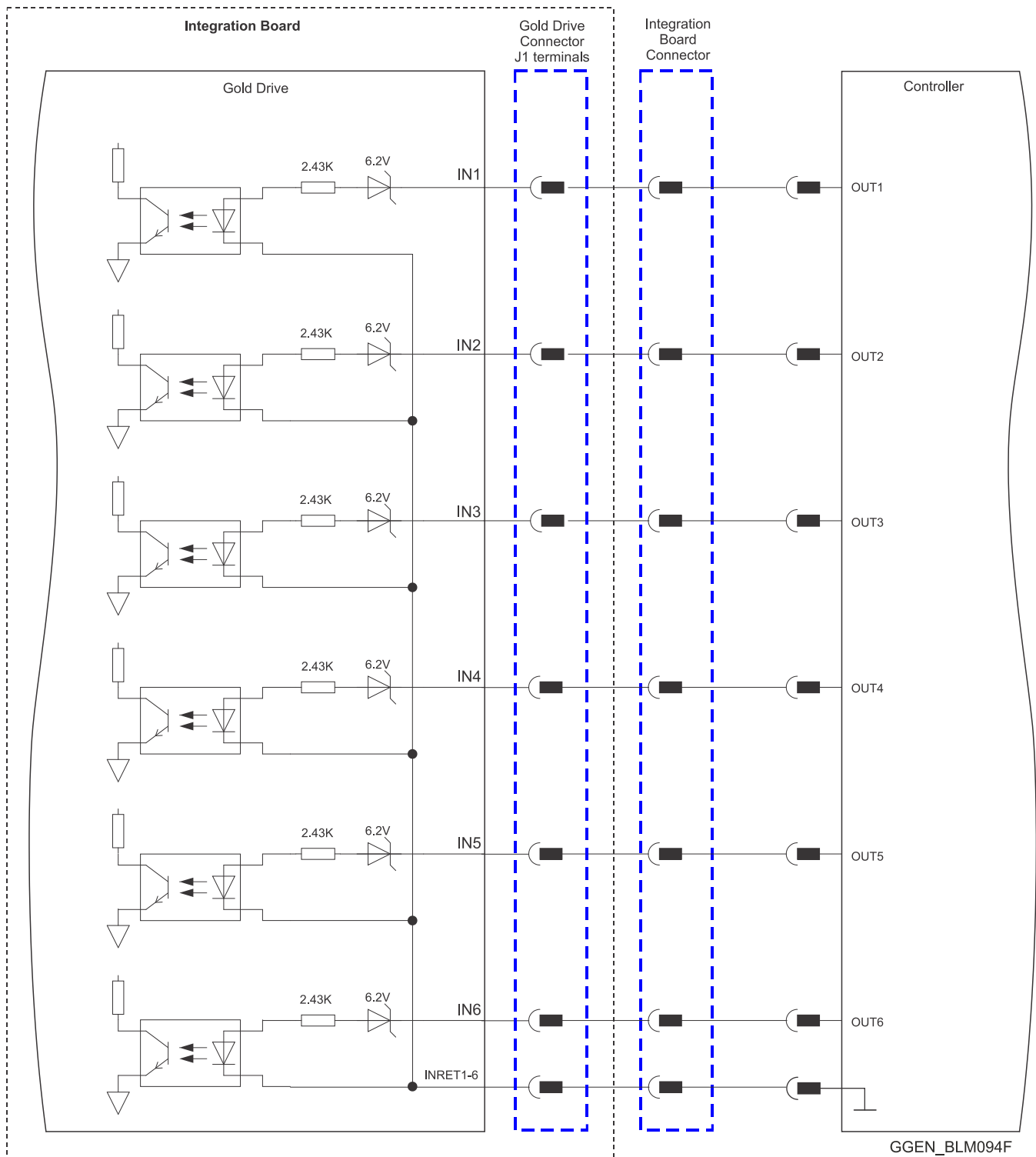
Figure 46: Digital Input Source Mode - PLC voltage level Connection Diagram
