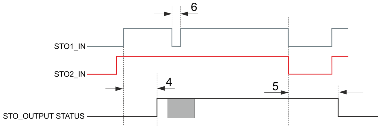
Figure 23: STO Out Signal Time
