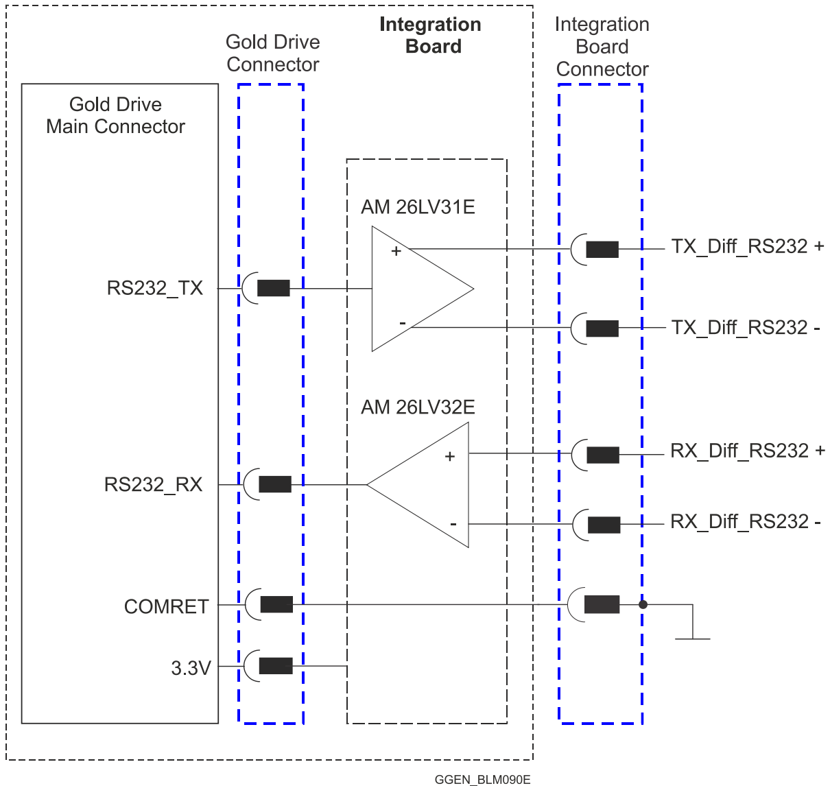
Figure 65: Differential RS232 Interfacing
