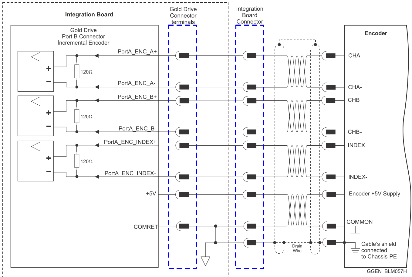
Figure 32: Port B Incremental Encoder Input – Recommended Connection Diagram
