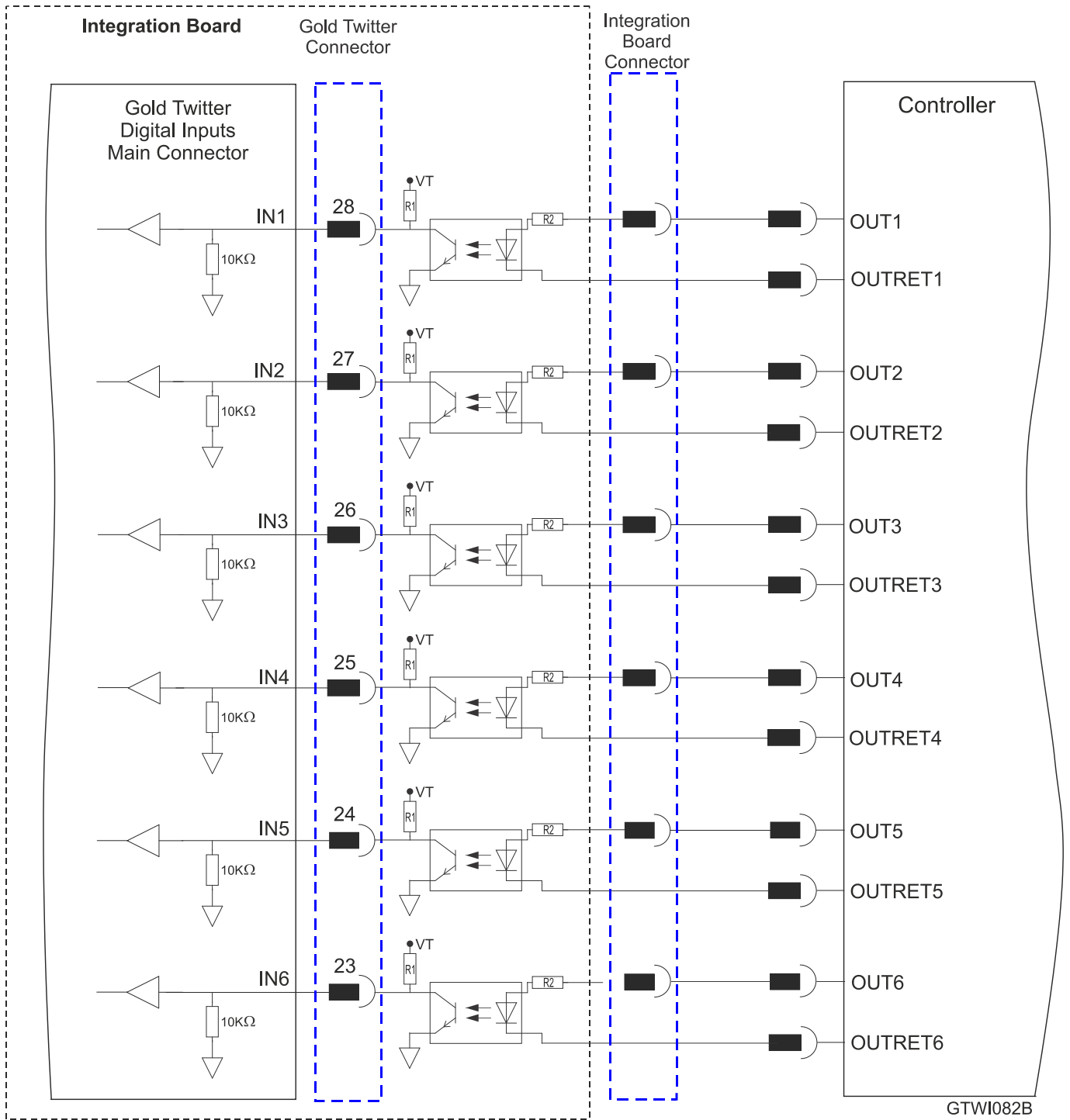
Figure 51: Digital Input 5V Logic level Mode Connection Diagram
