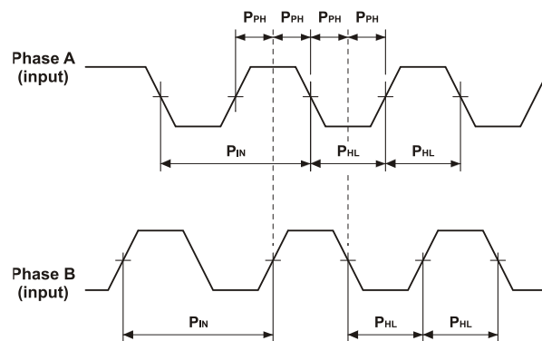
Figure 31: Main Feedback - Encoder Phase Diagram
