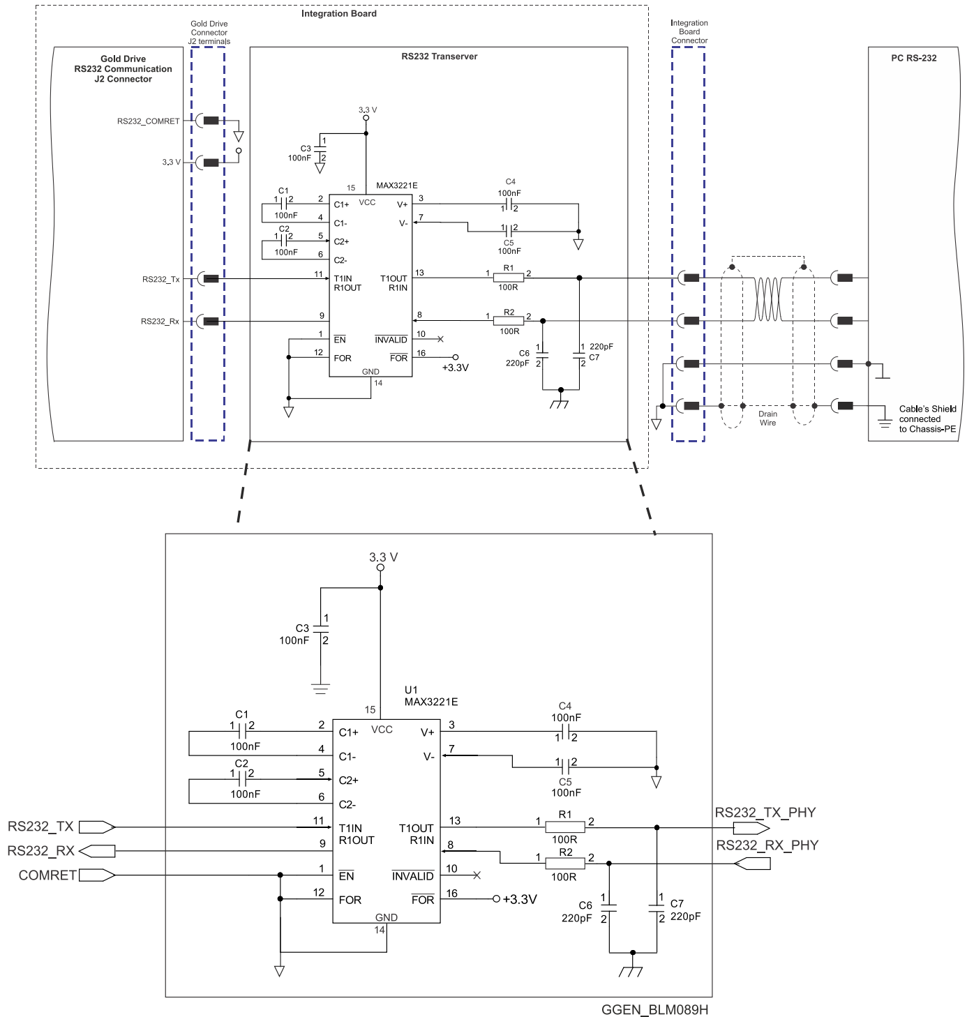
Figure 64: Standard RS232 Voltage Level incorporating RS232 TX/RX Transceiver Connection Diagram
