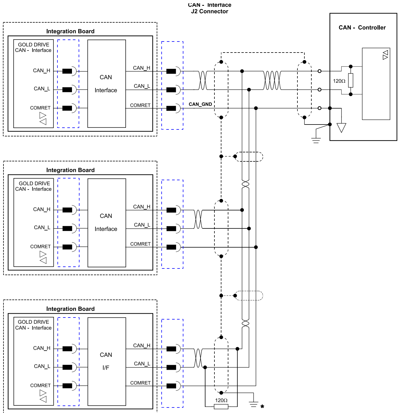
Figure 62: CANbus Connections
