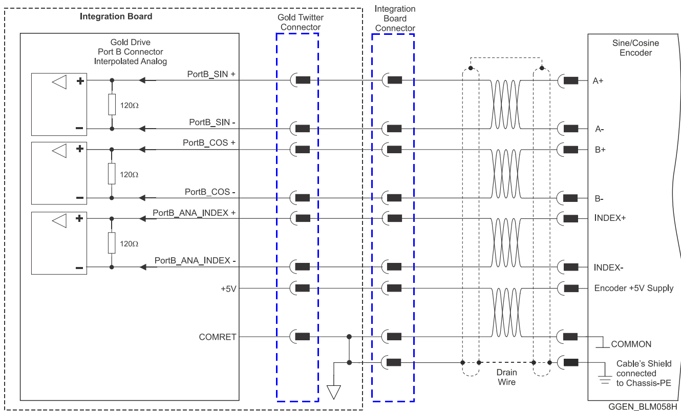
Figure 33: Port B - Interpolated Analog Encoder Connection Diagram
