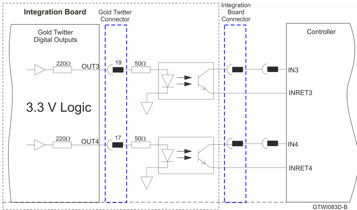
Figure 53: Digital Output 3.3V Logic Mode Connection Diagram
