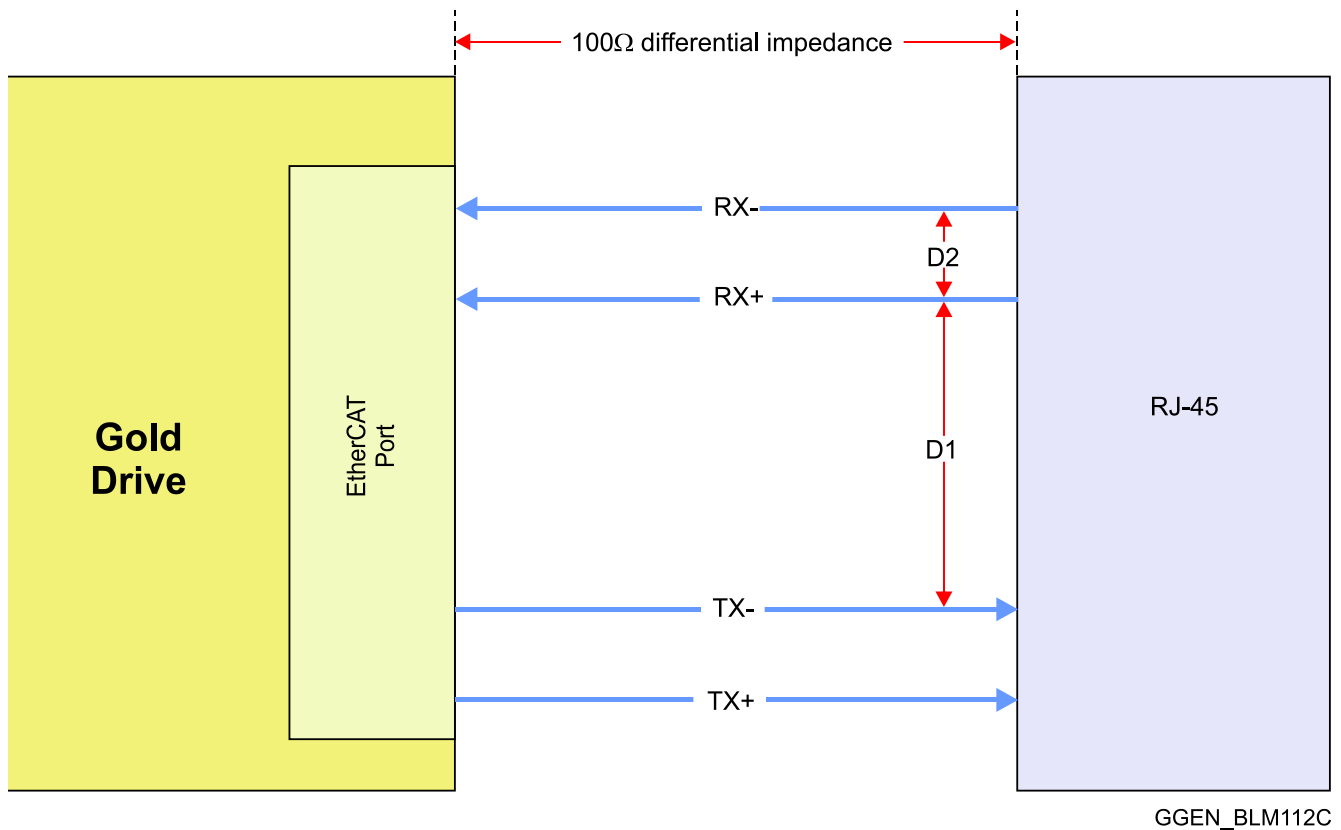
Figure 61: Differential Signal Layout
