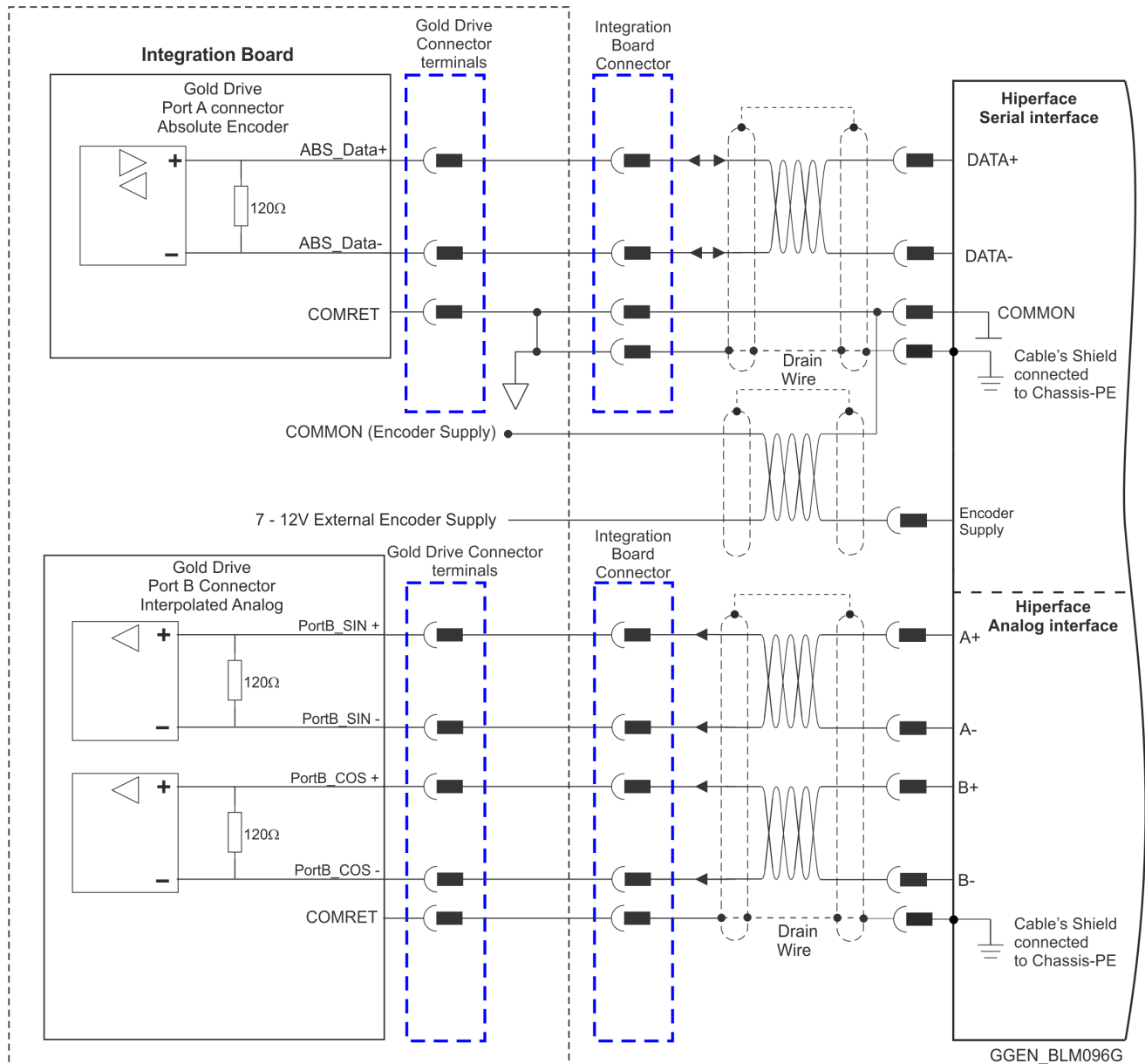
Figure 30: Absolute Serial Encoder – Recommended Connection Diagram for Stegmann Hiperface
