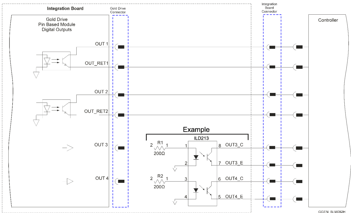
Figure 42: Digital Output Connection Diagram – TTL Connection
