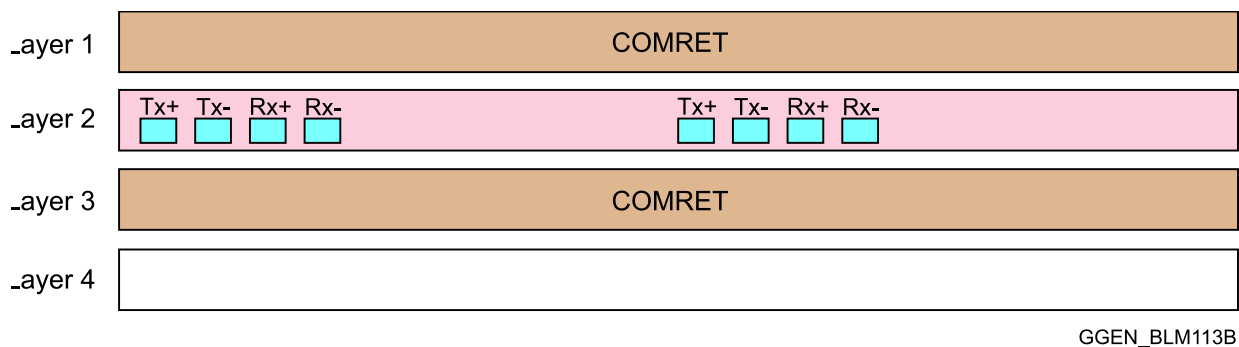
Figure 60: Example of Layered Stackup on PCB
