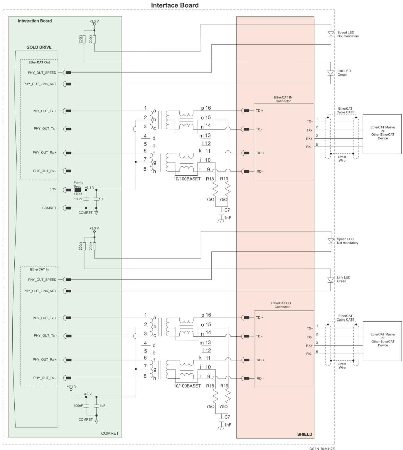
Figure 58: EtherCAT Connection Schematic without Magnetic Diagram
