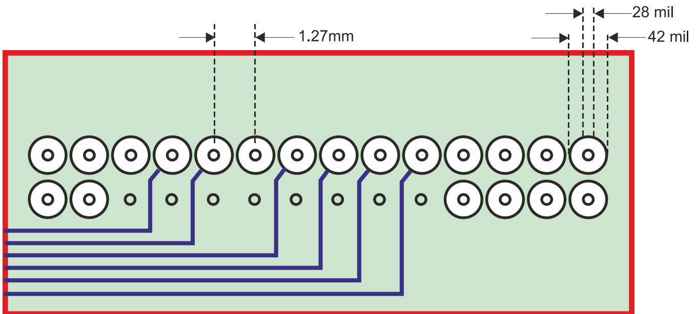
Figure 4: Routing the Trace between Pins
