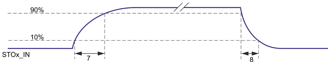
Figure 24: STO Rise and Fall Time
