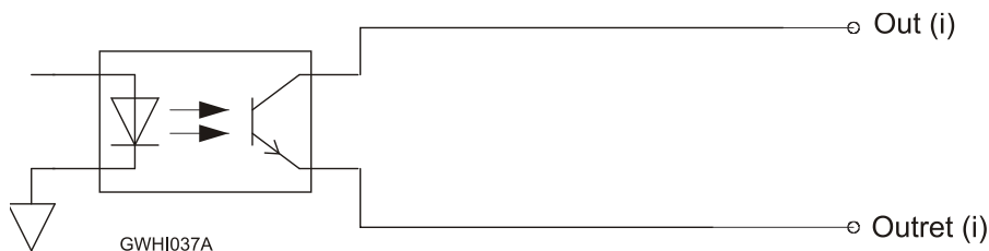
Figure 41: Digital Output Schematic
