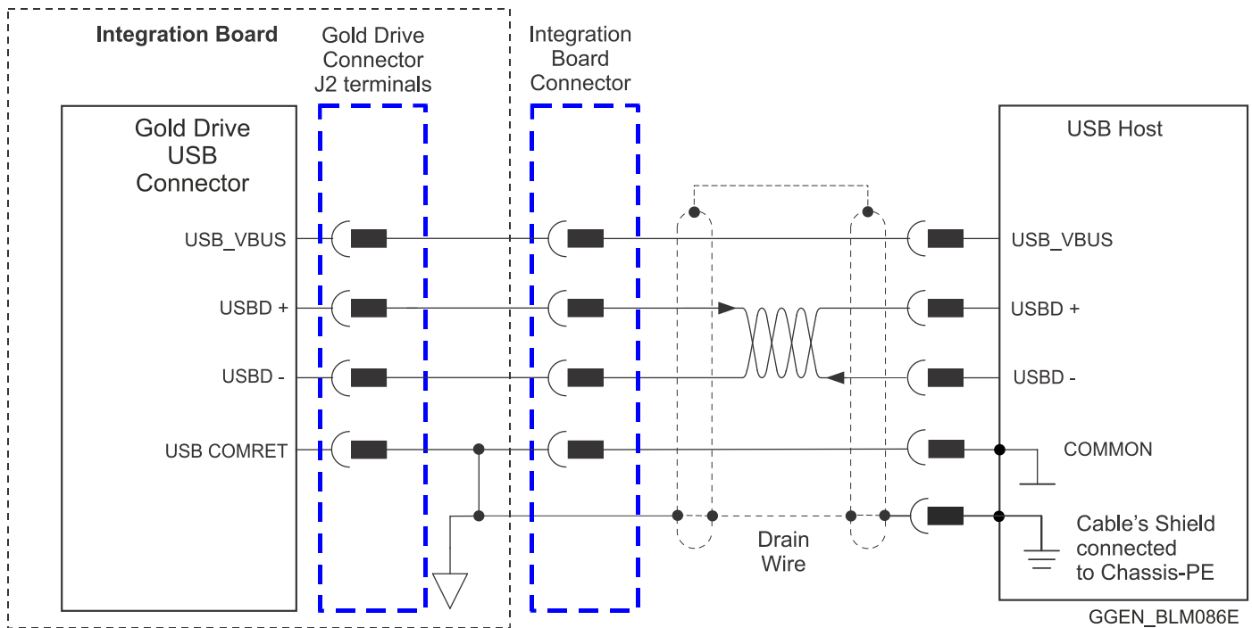
Figure 56: USB Network Diagram
