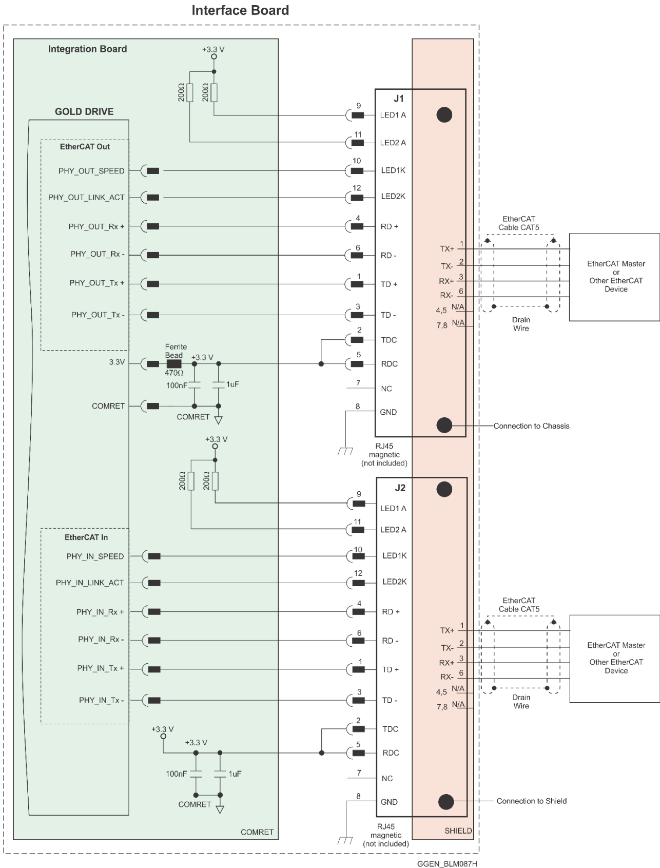
Figure 57: EtherCAT Connection Schematic with Diagram Sign of 3.3V
