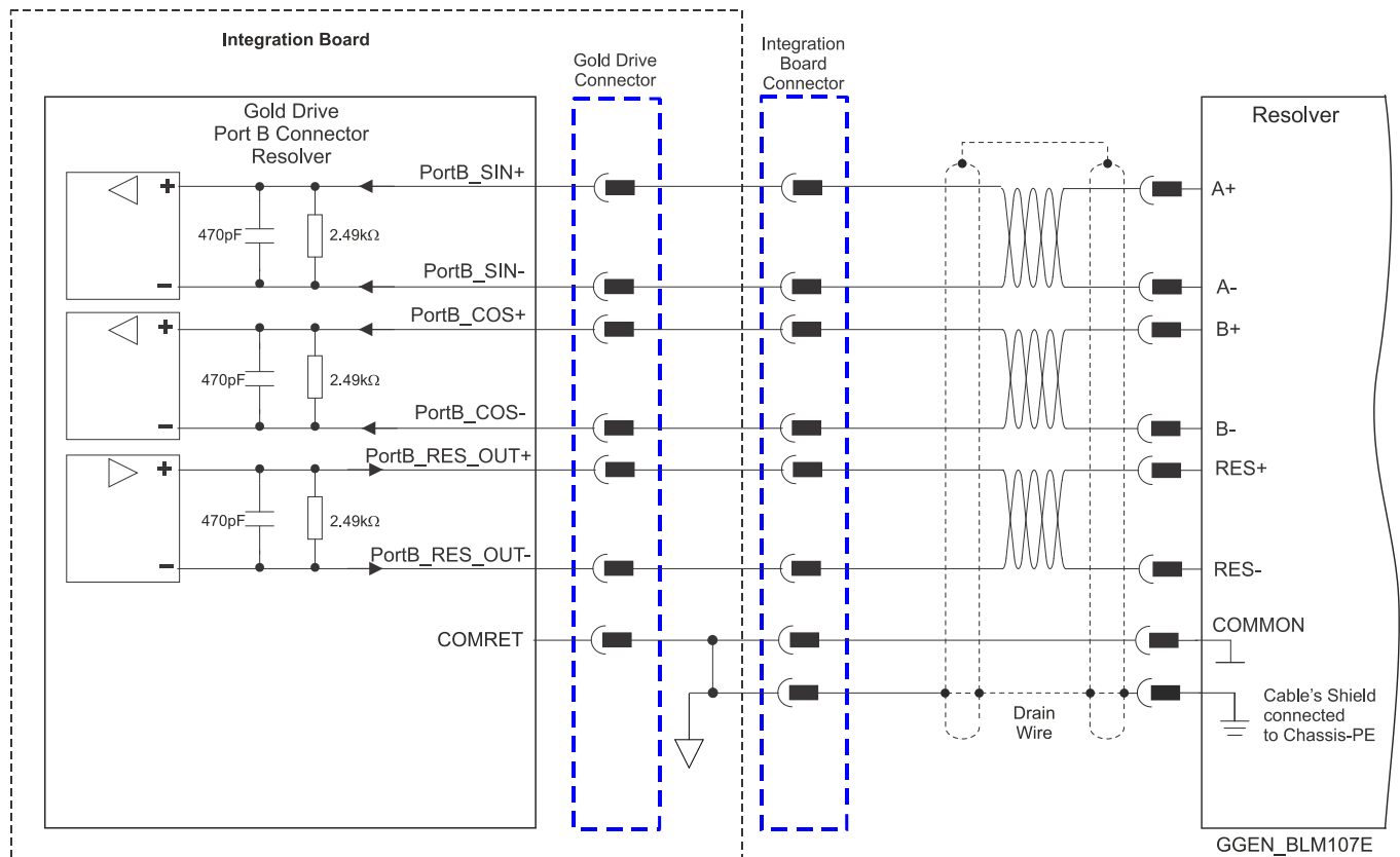
Figure 34: Port B – Resolver Connection Diagram
