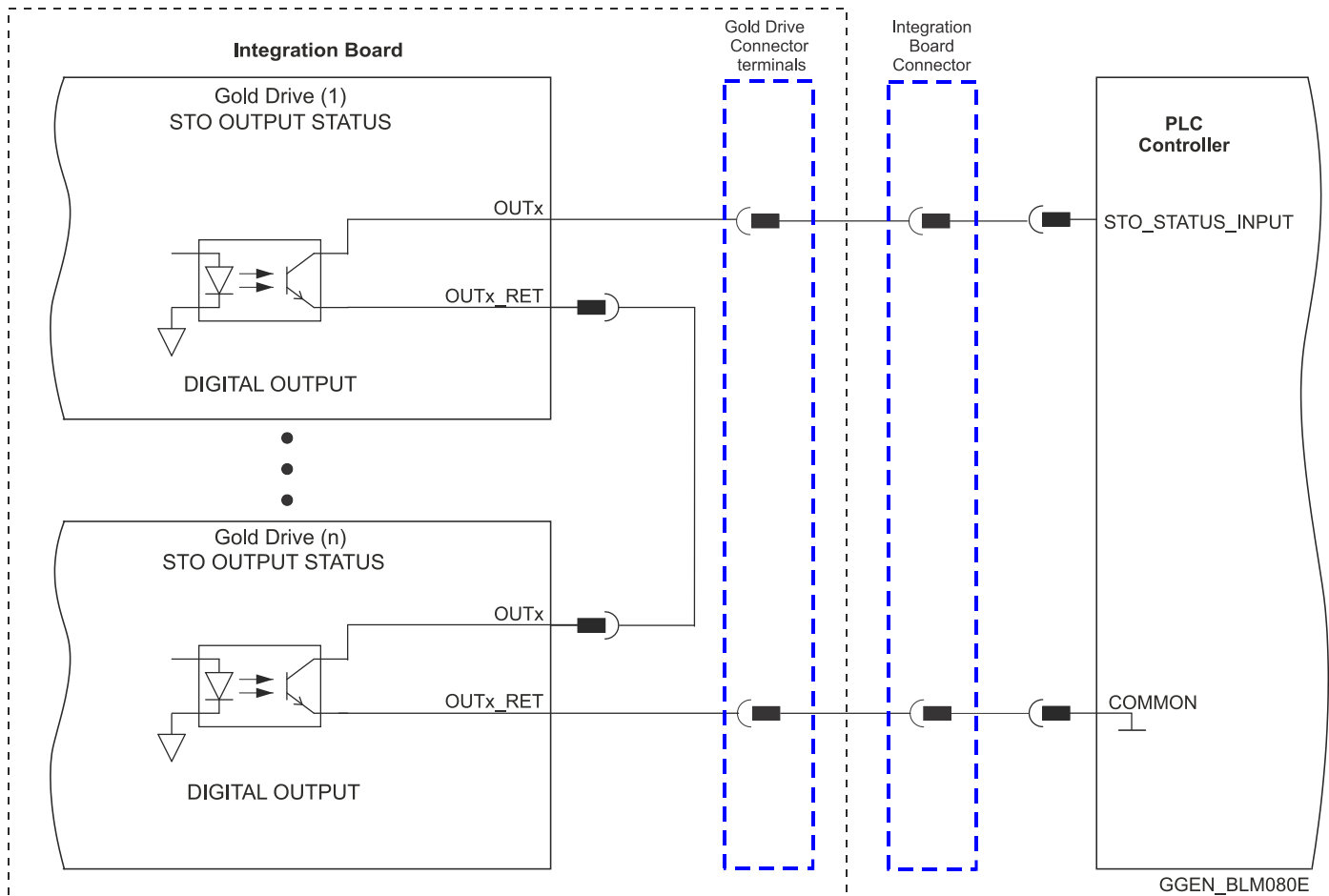
Figure 21: STO Dedicated Output Status
