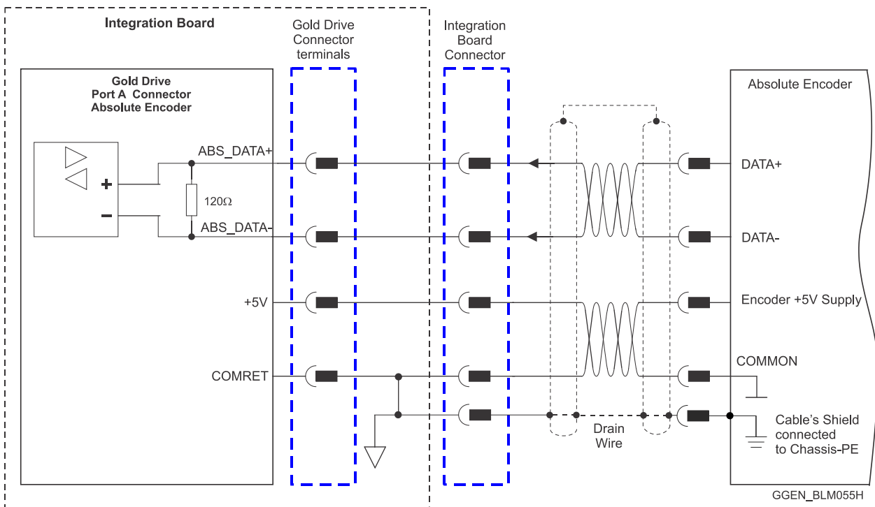
Figure 29: Absolute Serial Encoder – Recommended Connection Diagram for Panasonic, Tamgawai, Sanyo / Nikon
