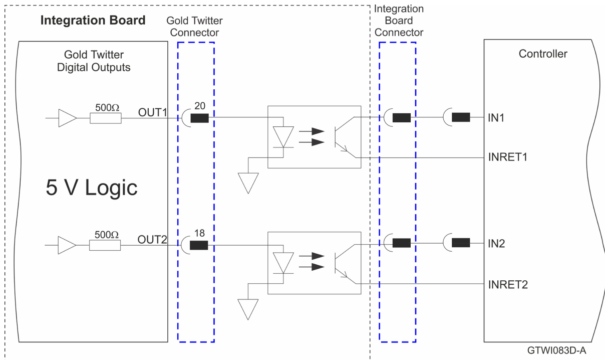
Figure 52: Digital Output 5V Logic Mode Connection Diagram
