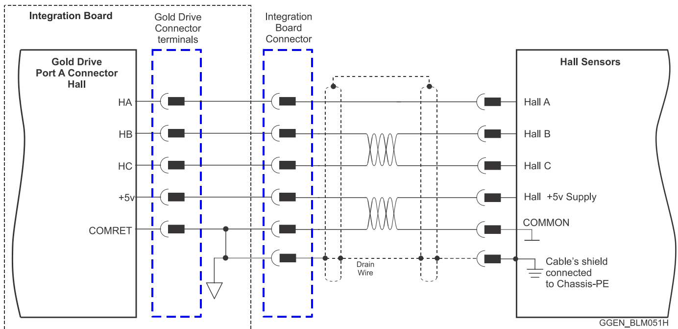
Figure 27: Hall Sensors Connection Diagram
