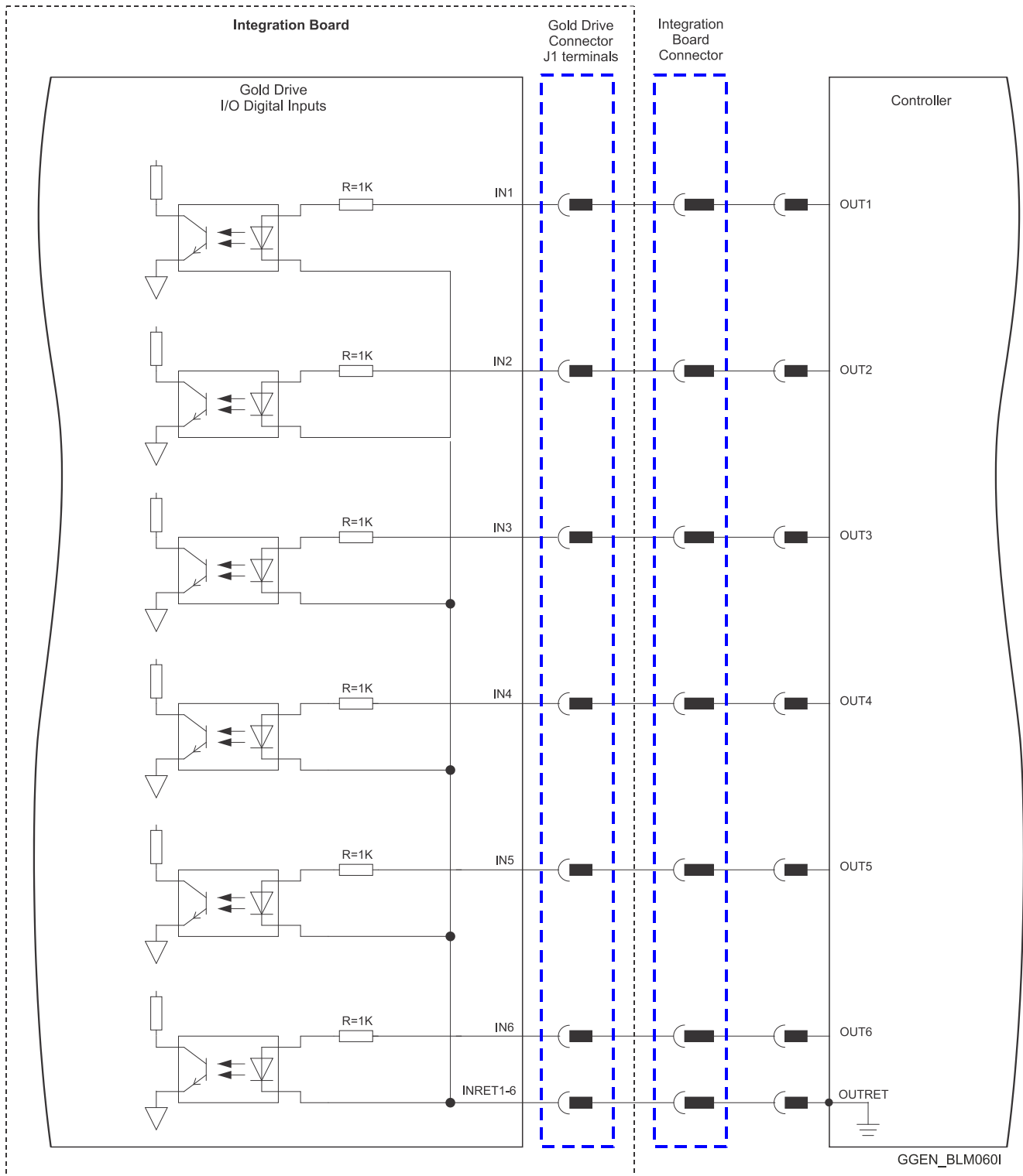
Figure 44: Digital Input TTL Mode Connection Diagram
