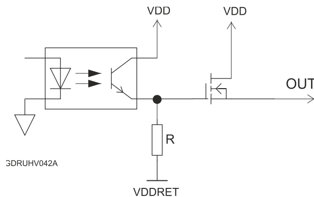
Figure 49: Digital Output Schematic – Source Mode PLC Level
