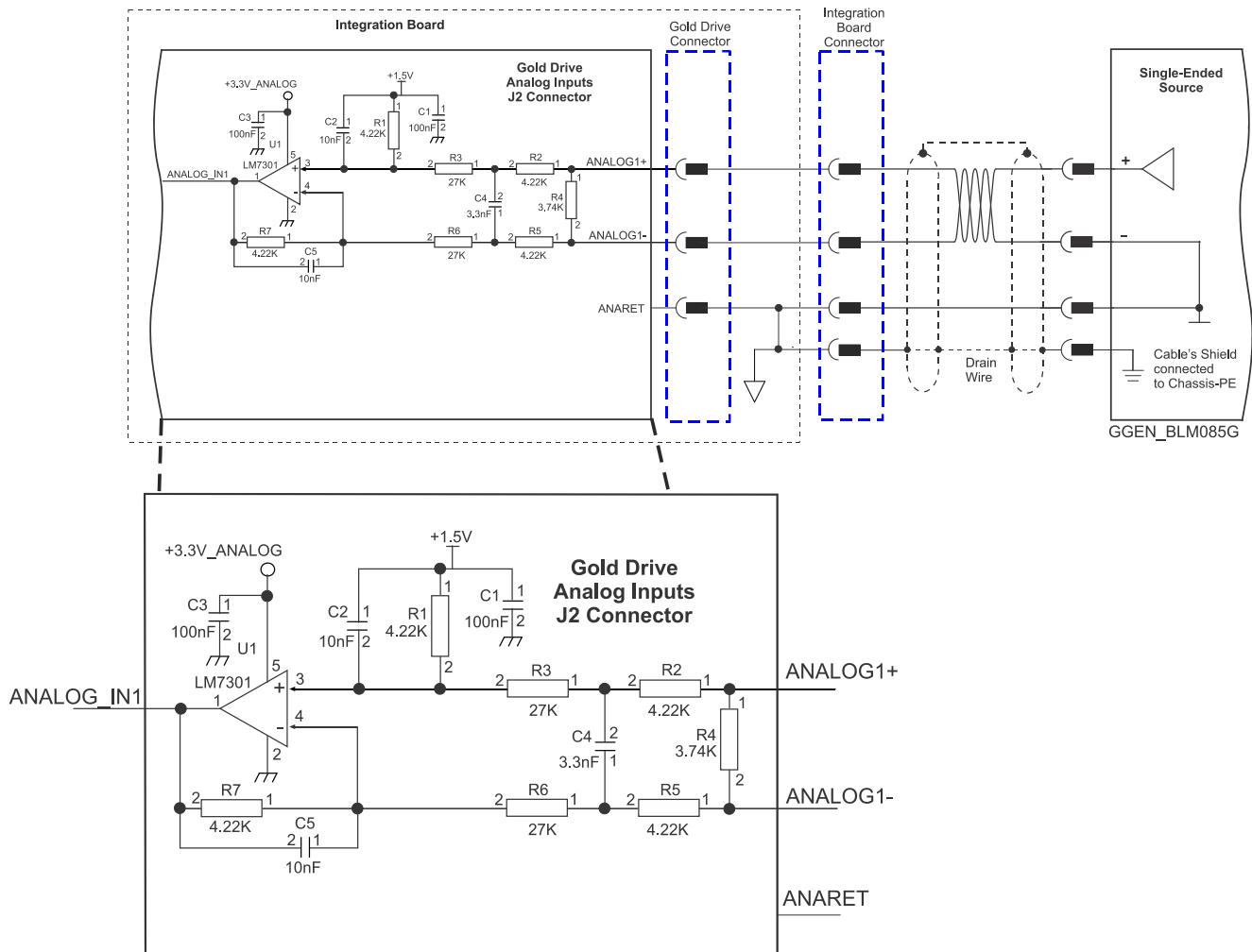
Figure 54: Analog Input with Differential -Ended Source
