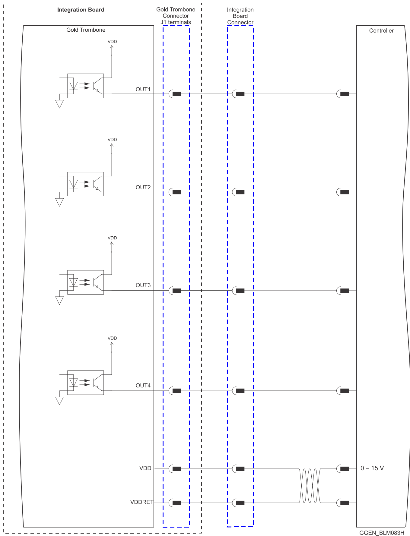
Figure 48: Digital Output Connection Diagram
