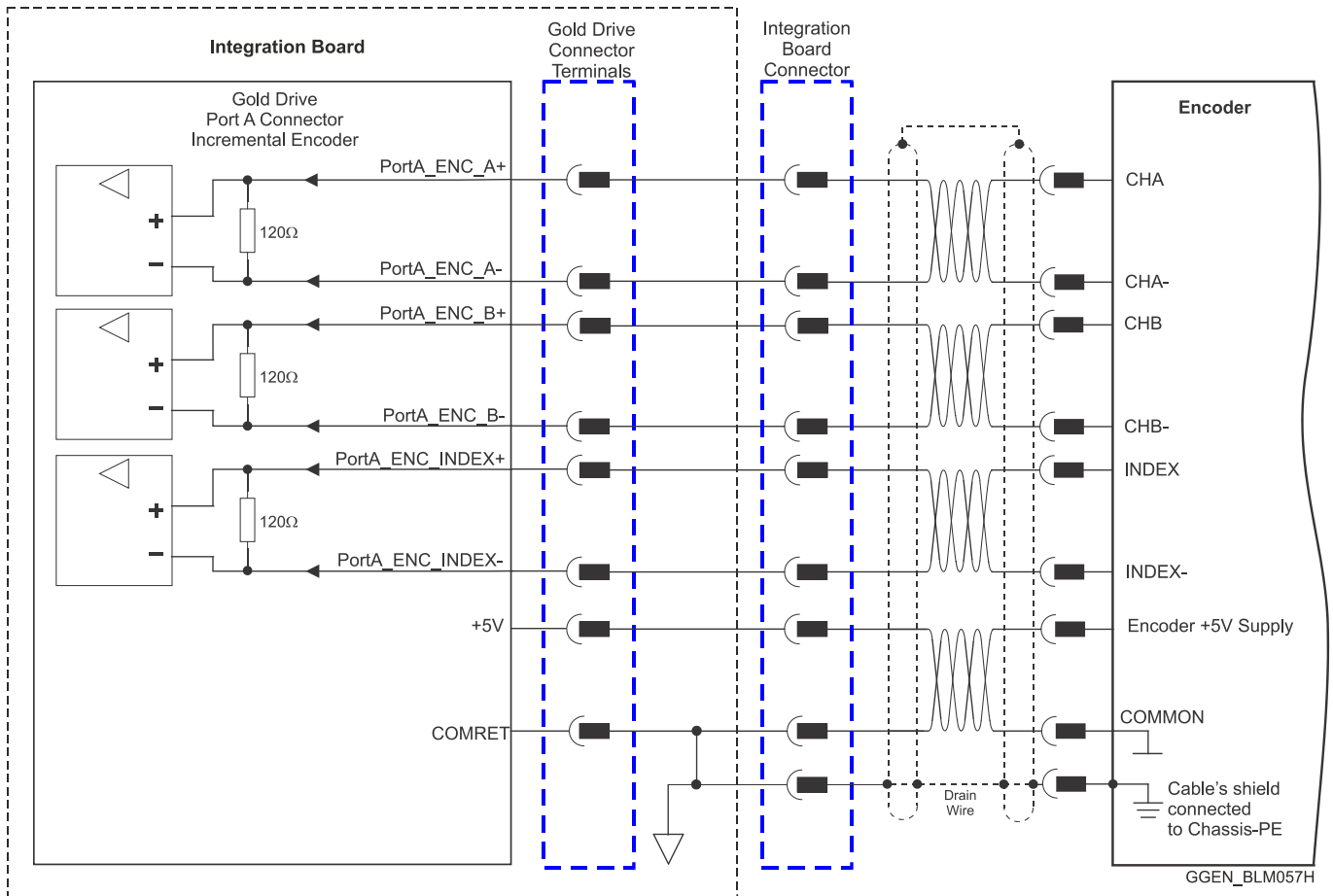
Figure 26: Port A Incremental Encoder Input – Recommended Connection Diagram
