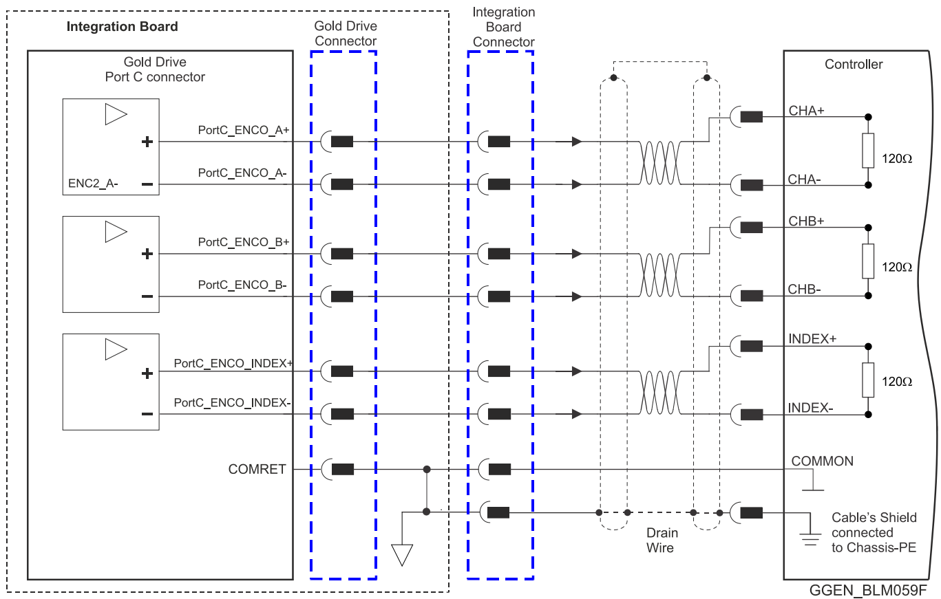
Figure 35: Emulated Encoder Differential Output – Recommended Connection Diagram
