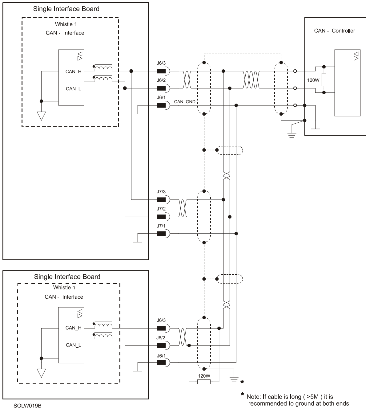
Figure 23: CANopen Network Diagram
