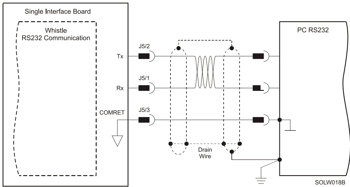
Figure 22: RS-232 Connection Diagram
