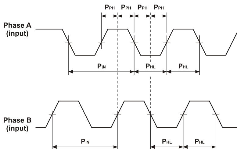
Figure 24: Main Feedback - Encoder Phase Diagram
