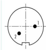
FACE VIEW 99 0071 100 02
