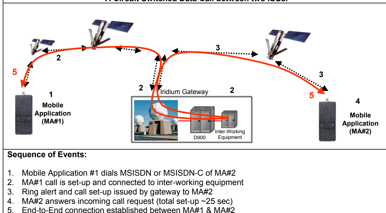
Figure 2 A Circuit Switched Data Call between two ISUs.
