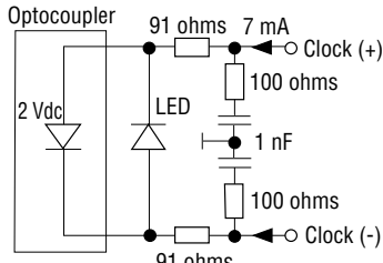
Figure 1. Sensor input
