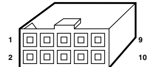
10 POSITION IDC CONNECTOR CENTER POLARIZED.
