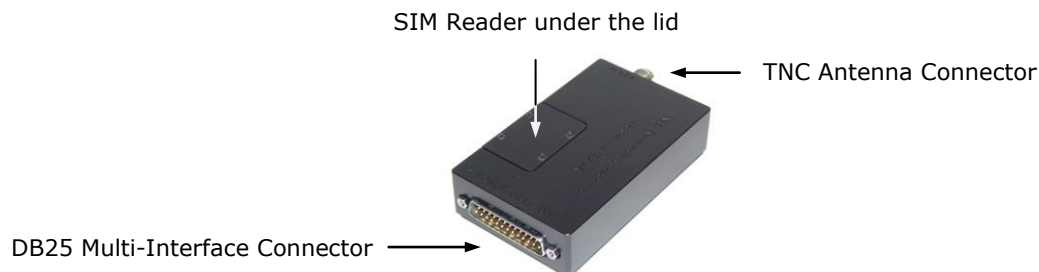
Figure 1. Iridium Satellite Modem A3LA-R.
