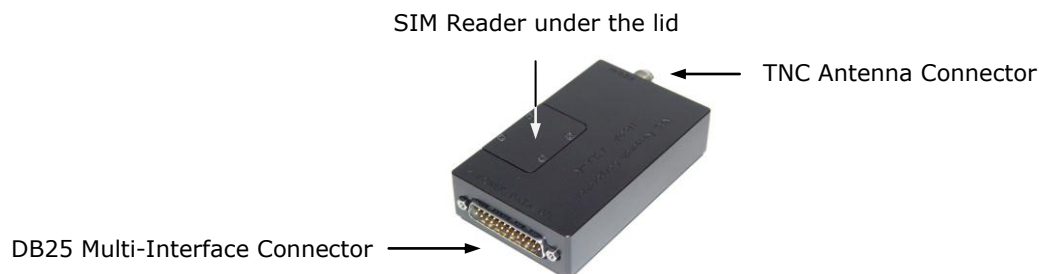
Figure 1. Iridium Satellite Modem A3LA-RM.
