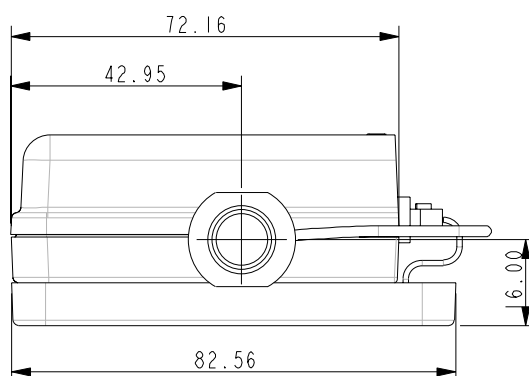
Figure 11: End View
