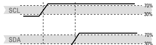
Figure 14 Transmission Stop condition (P) - a low to high transition on the SDA line while SCL is high. The Stop condition is a unique state on the bus created by the master, indicating to the slaves the end of a transmission sequence (bus is considered free after a Stop).
