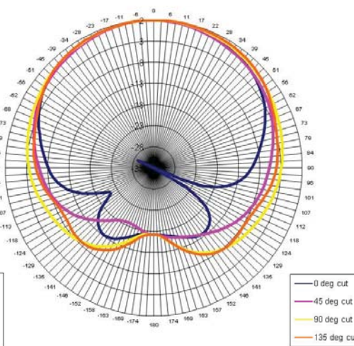
Elevation Plot
