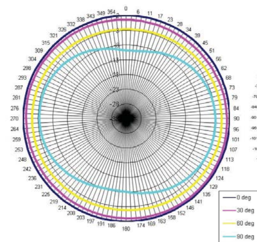
Azimuth Plot
