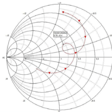
Impedance Plot
