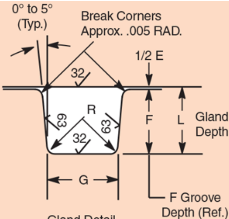
Gland Detail
