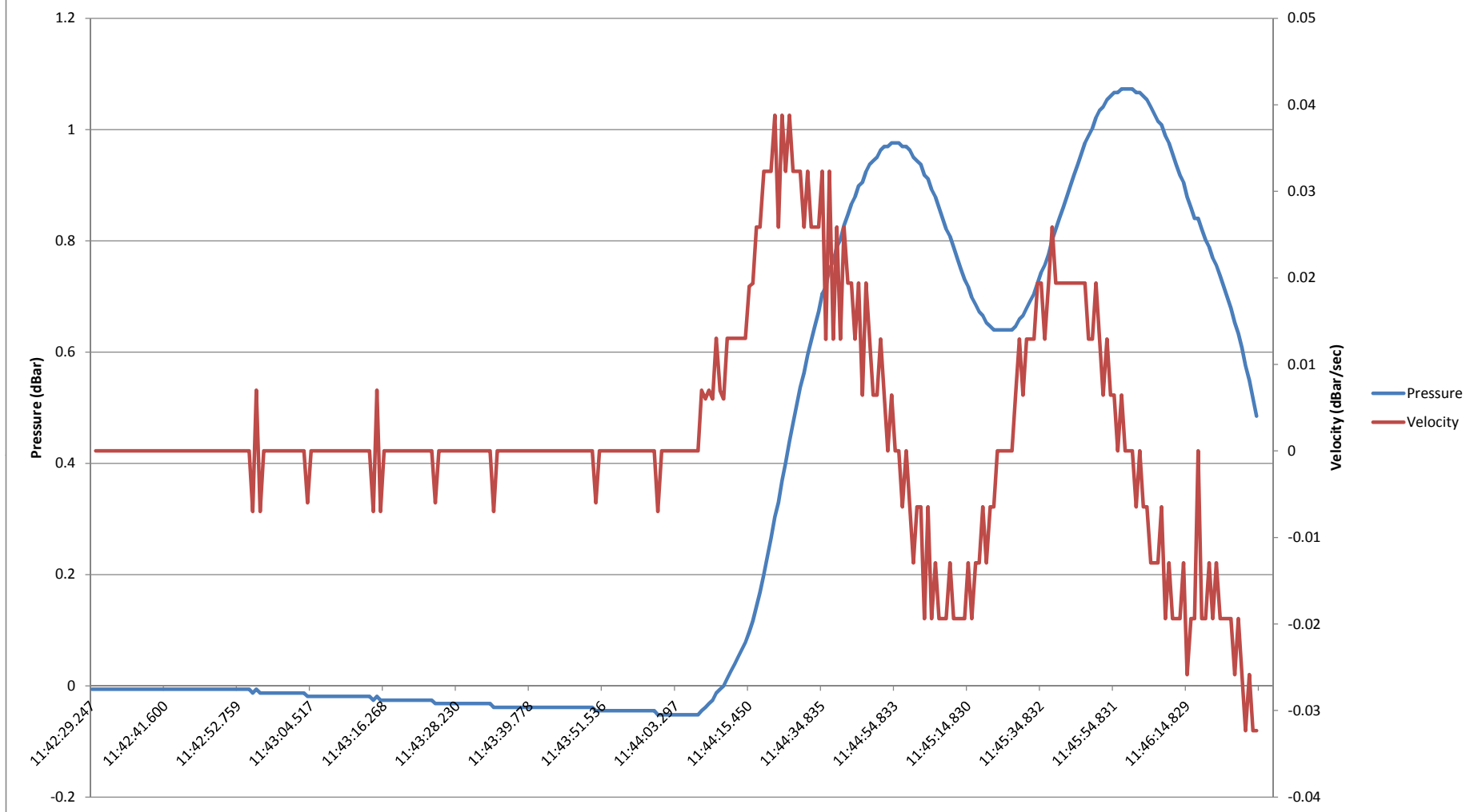
CPF Profile Under Velocity Control
