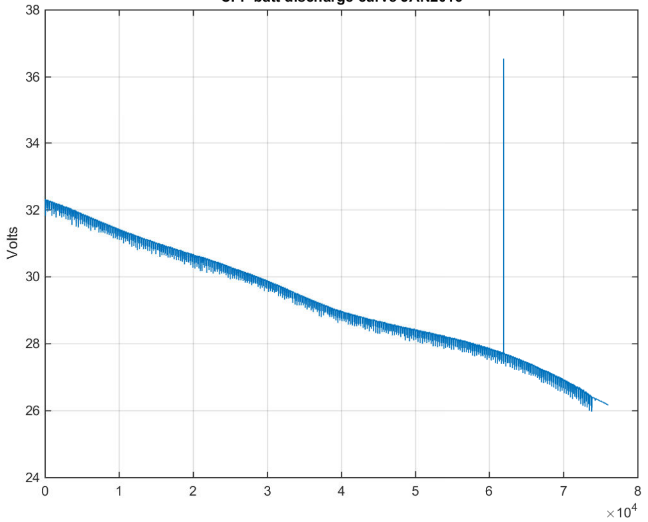
CPF batt discharge curve JAN2016
