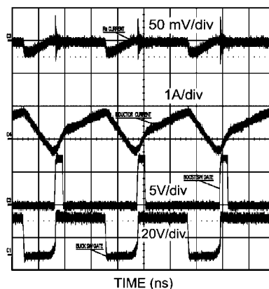
FIGURE 5. Mode Transition
