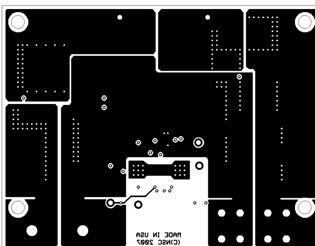
Bottom Layer as Viewed from Top
