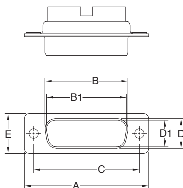
TYPICAL CONNECTOR TOP VIEW
