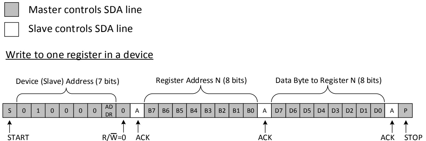
Figure 26. Write to Register
