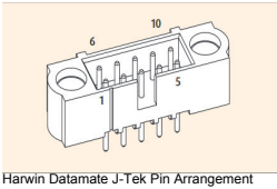
Harwin Datamate J-Tek Pin Arrangement
