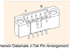
Harwin Datamate J-Tek Pin Arrangement
