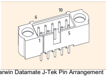
Harwin Datamate J-Tek Pin Arrangement
