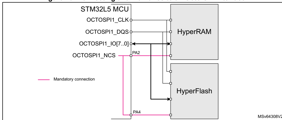
Figure 10. Connecting two memories to an Octo-SPI interface
