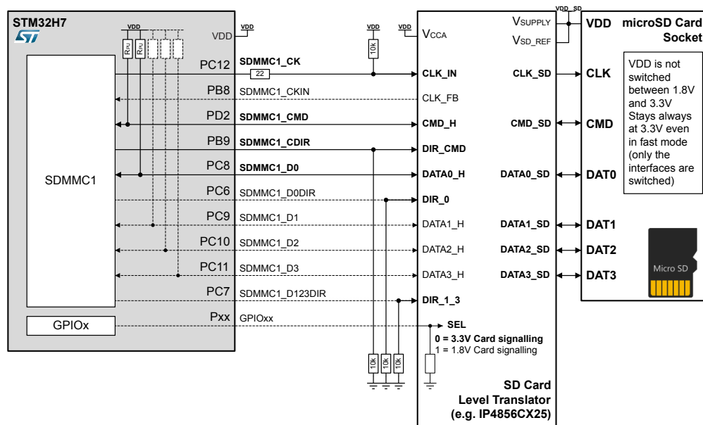
Figure 24. µSDCard interconnection example
