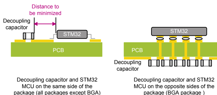
Figure 22. Decoupling capacitor placement depending on package type
