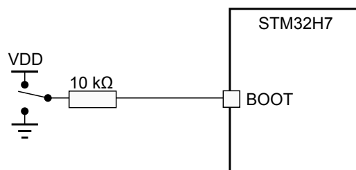
Figure 16. Boot mode selection implementation example
