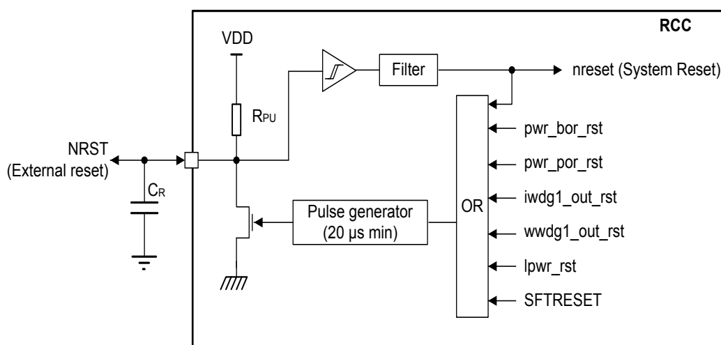
Figure 10. Reset circuit
