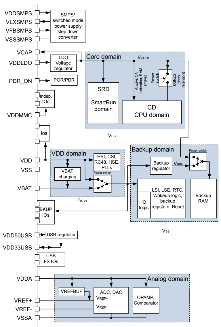
Figure 1. Power supplies
