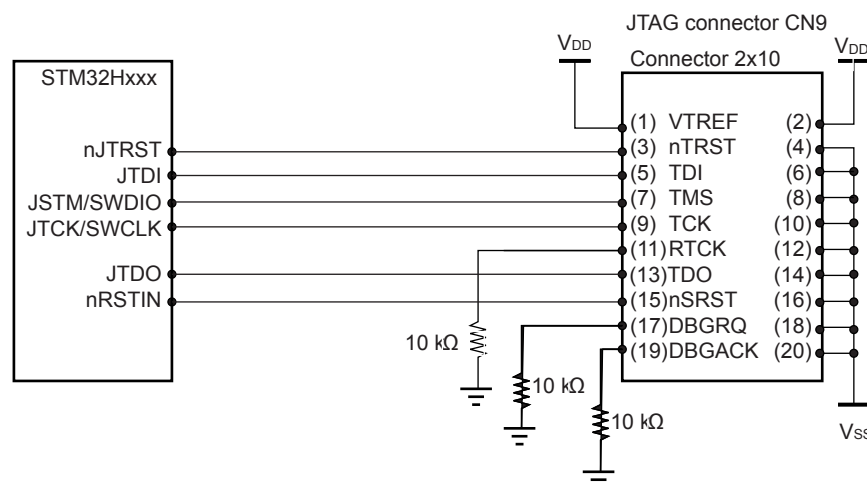
Figure 18. JTAG connector implementation
