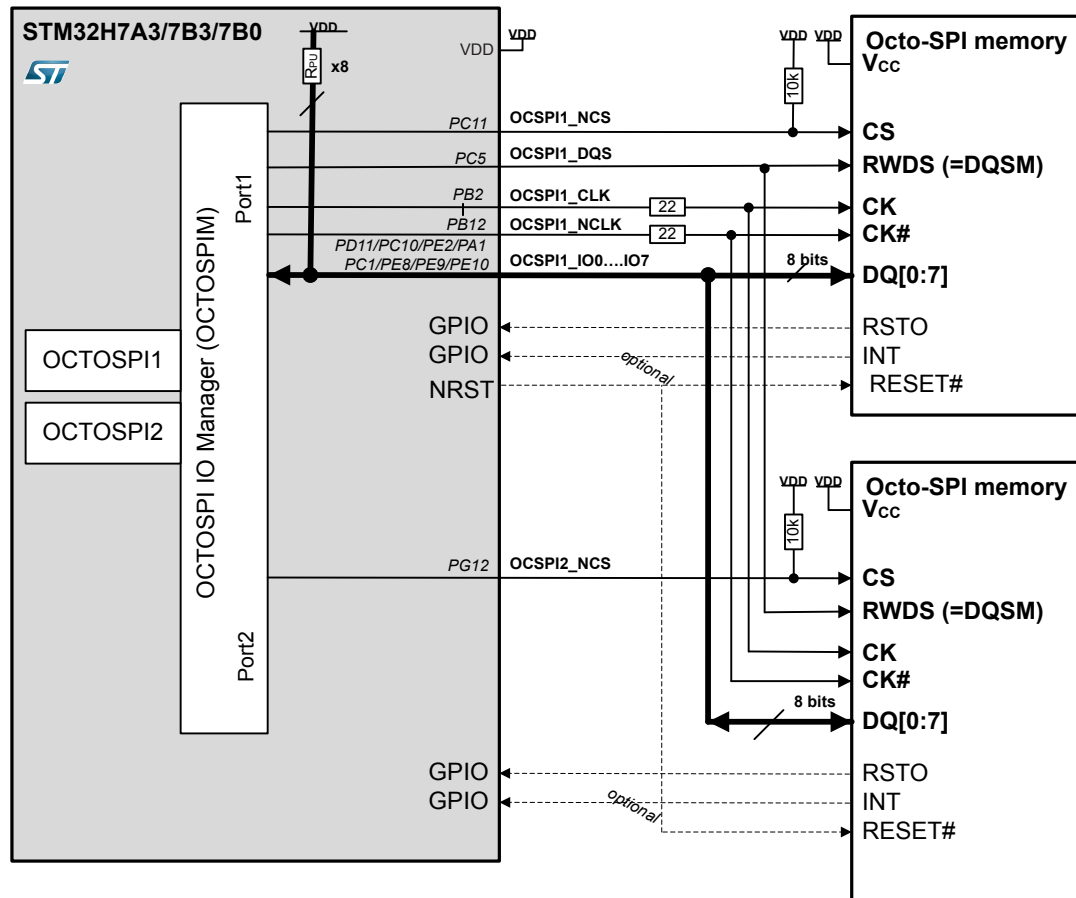
Figure 28. Octo-SPI multiplexed interconnection example
