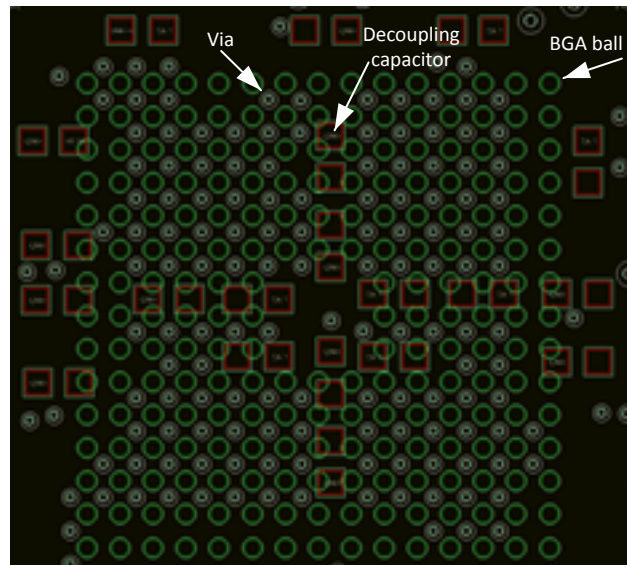
Figure 23. Example of decoupling capacitor placed underneath
