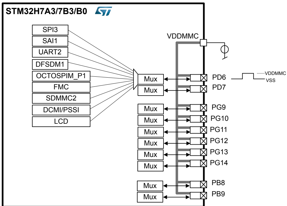
Figure 15. VDDMMC supplied pads
