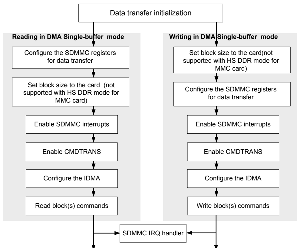
Figure 24. Read/write data in DMA Single-buffer mode
