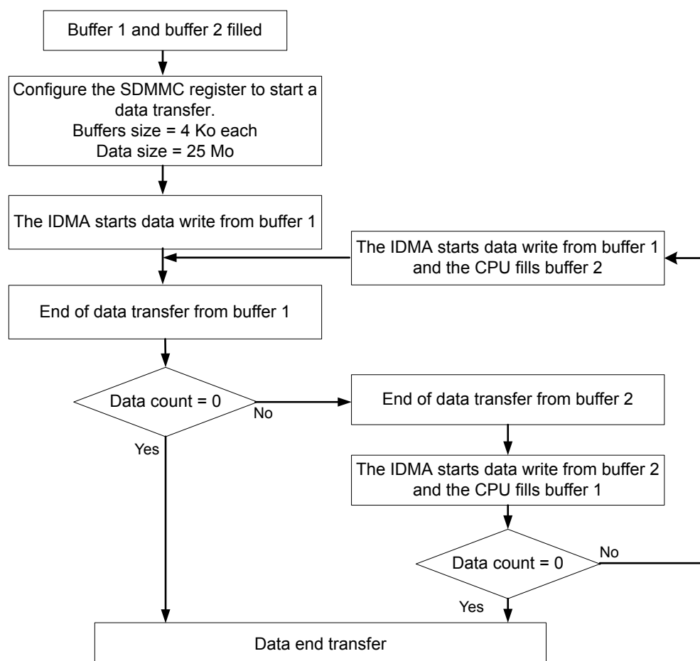
Figure 26. IDMA Double-buffer mode example
