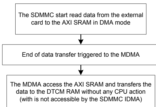
Figure 32. MDMA and SDMMC end of data transfer example
