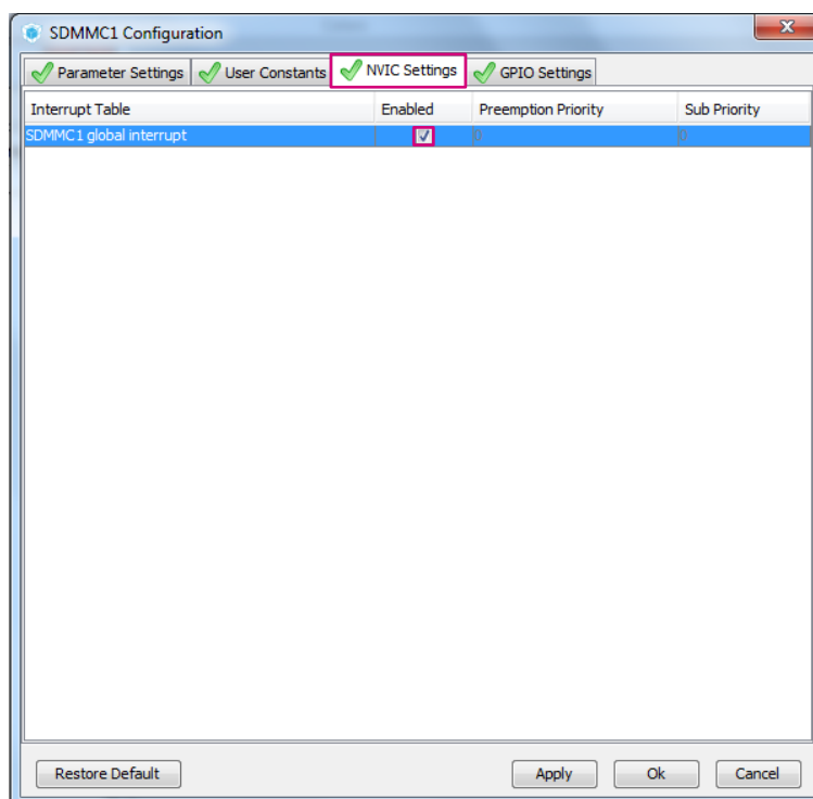
Figure 12. SDMMC global interrupt configuration with STM32CubeMx
