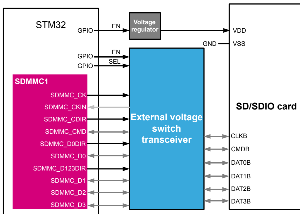
Figure 5. Voltage switch transceiver
