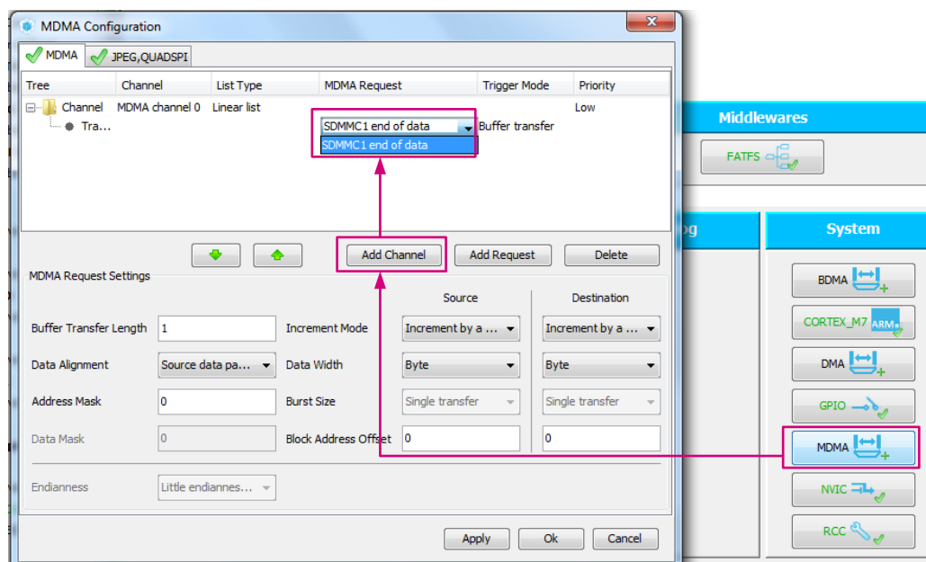
Figure 14. MDMA end of data configuration with STM32CubeMx
