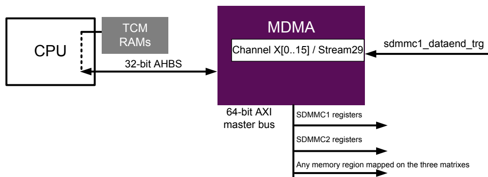
Figure 3. Master DMA (MDMA)
