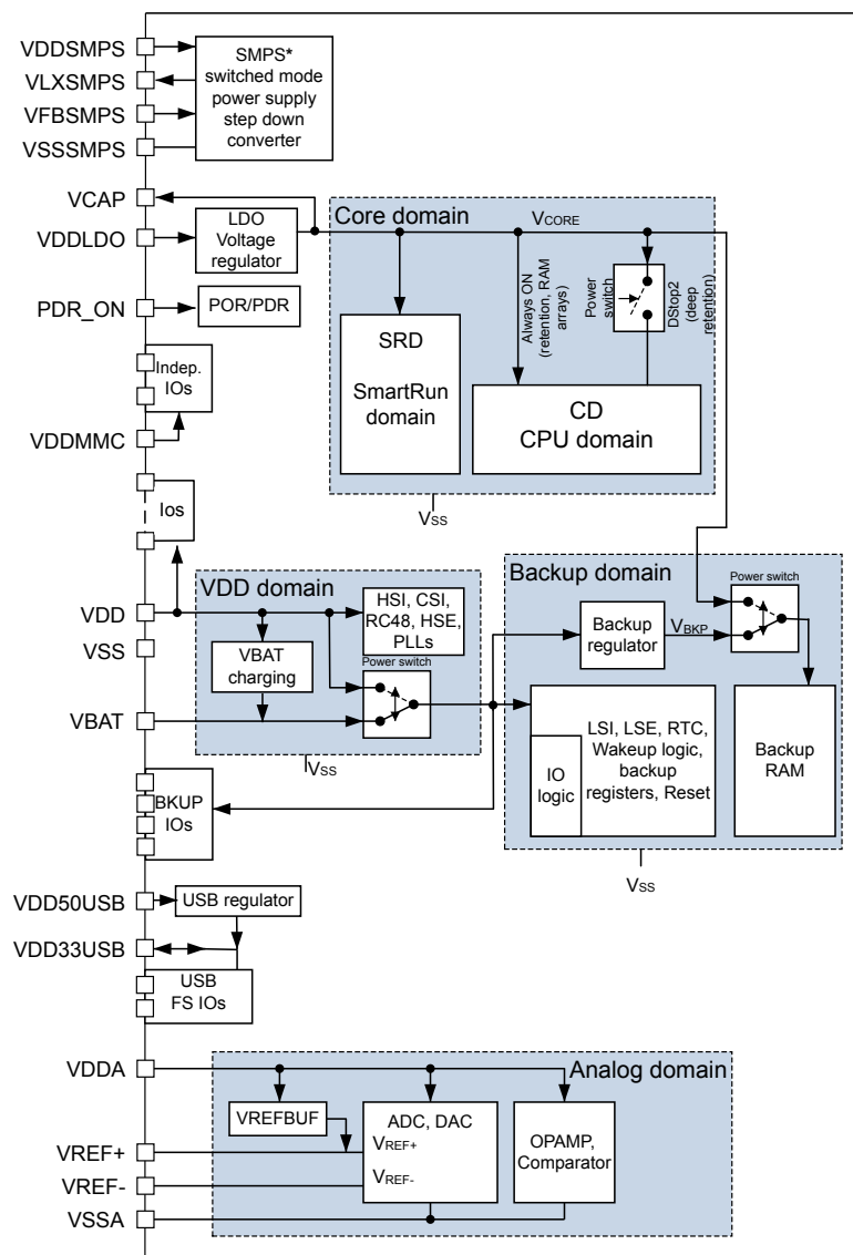
Figure 1. Power supplies
