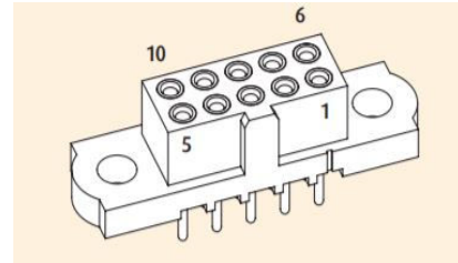
Harwin Datamate J-Tek Pin Arrangement -- Female
