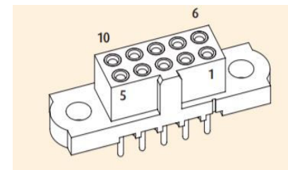
Harwin Datamate J-Tek Pin Arrangement -- Female
