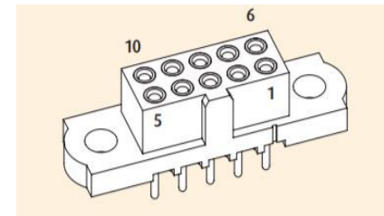
Harwin Datamate J-Tek Pin Arrangement -- Female
