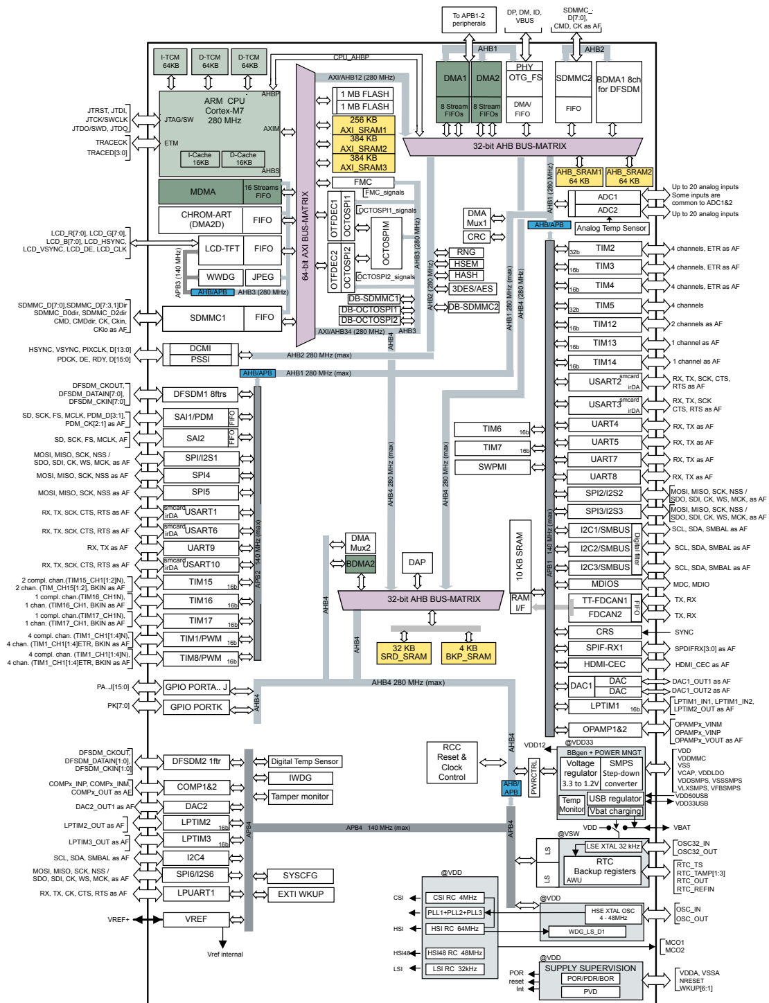
Figure 1. STM32H7B3xl block diagram
