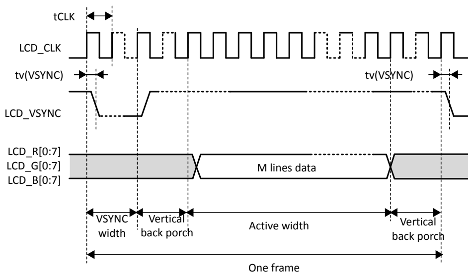
Figure 65. LCD-TFT vertical timing diagram
